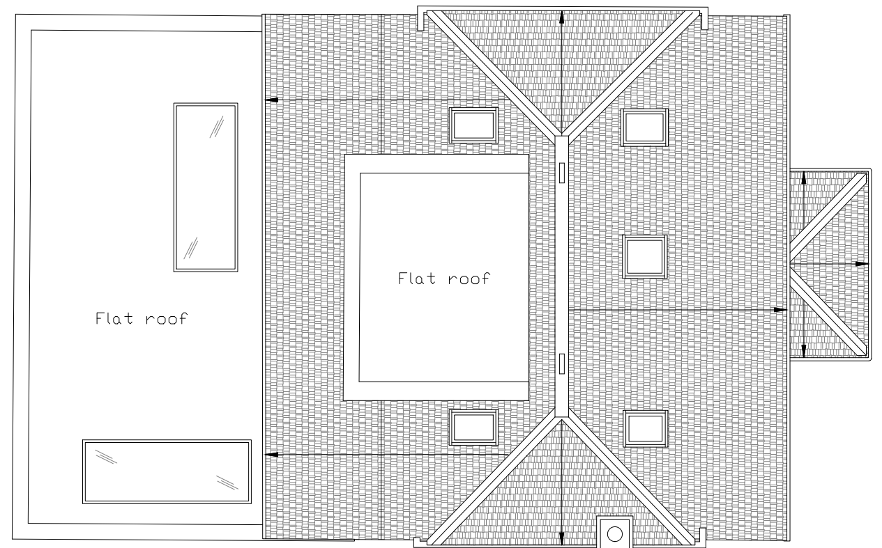
02 P(02)_101 Proposed Roof Plan 1:100@A3
