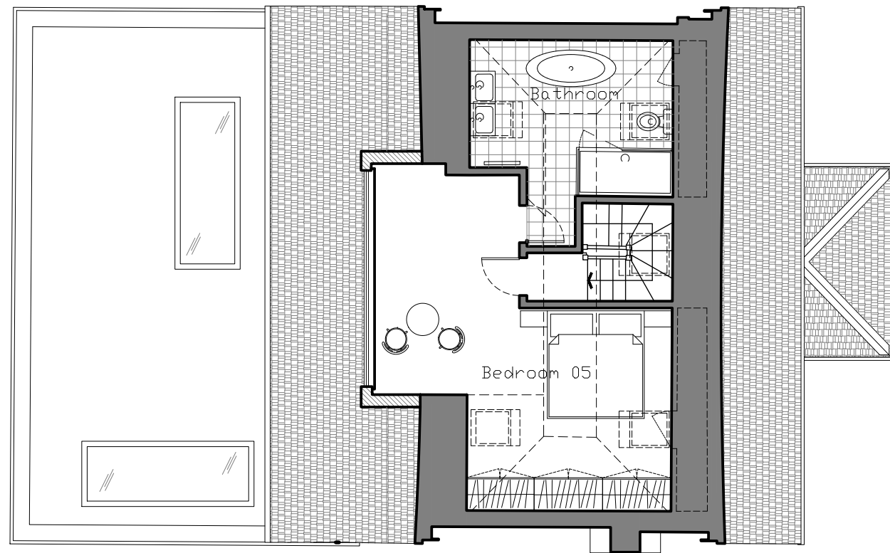
01 P(02)_101 Proposed Second Floor Plan 1:100@A3
