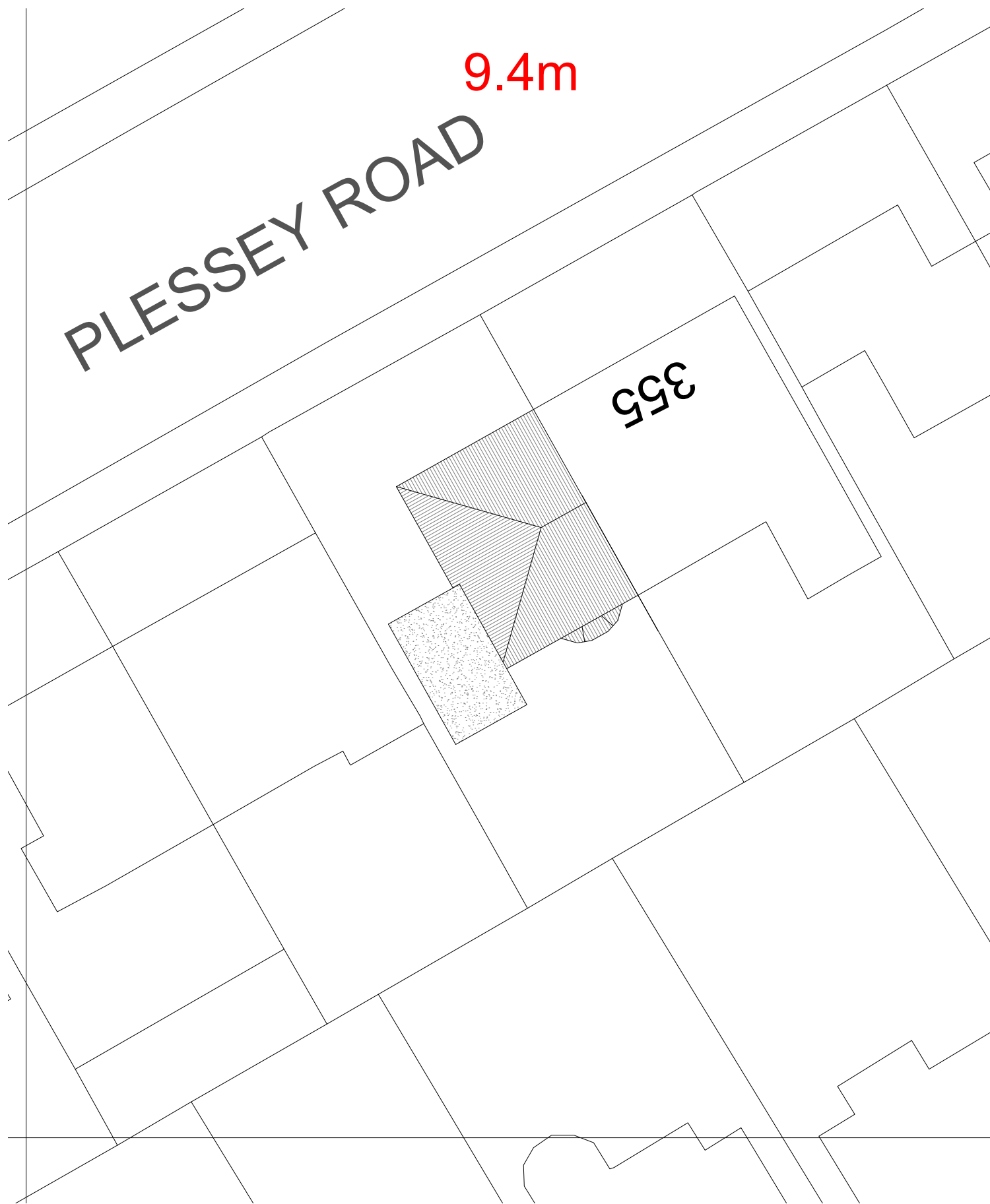
EXISTING BLOCK PLAN 1:200
