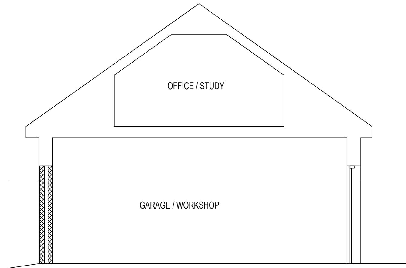
SECTION A-A AS PROPOSED 1:50
