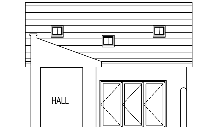
REAR ELEVATION AS PROPOSED 1:100
