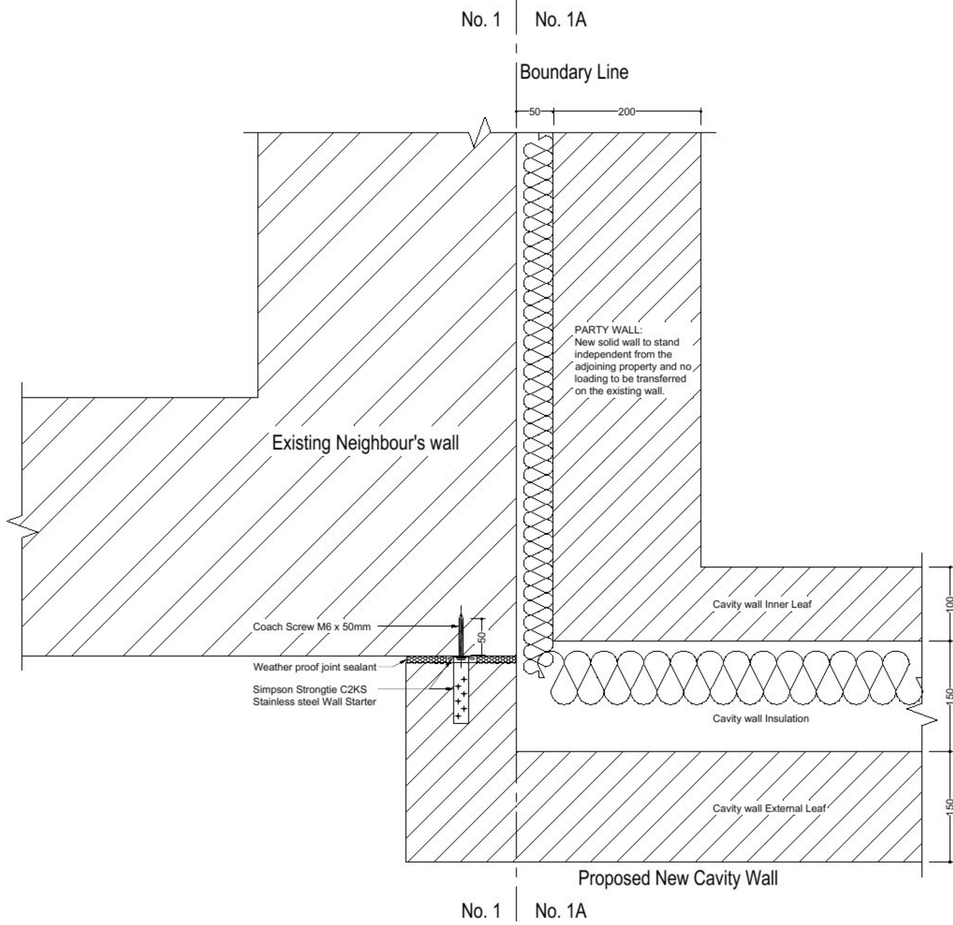
NEW WALL TO EXISTING WALL CONNECTION DETAIL PLAN "DETAIL A" 1:5
