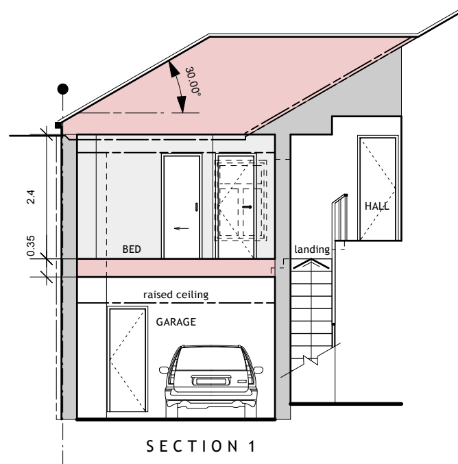
PROPOSED SECTIONS 1-3
