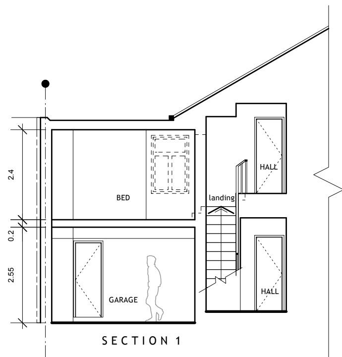
EXISTING SECTIONS 1-3
