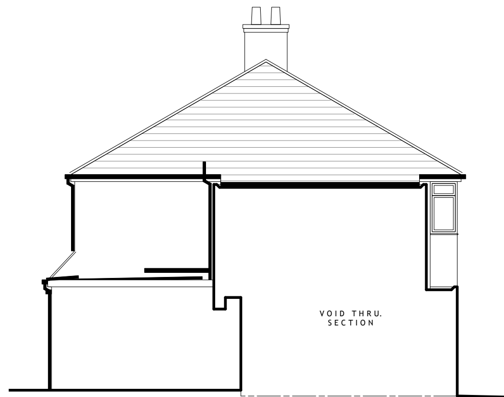
EXISTING SIDE ELEVATION CUT ALONG EXISTING SECTION 3
