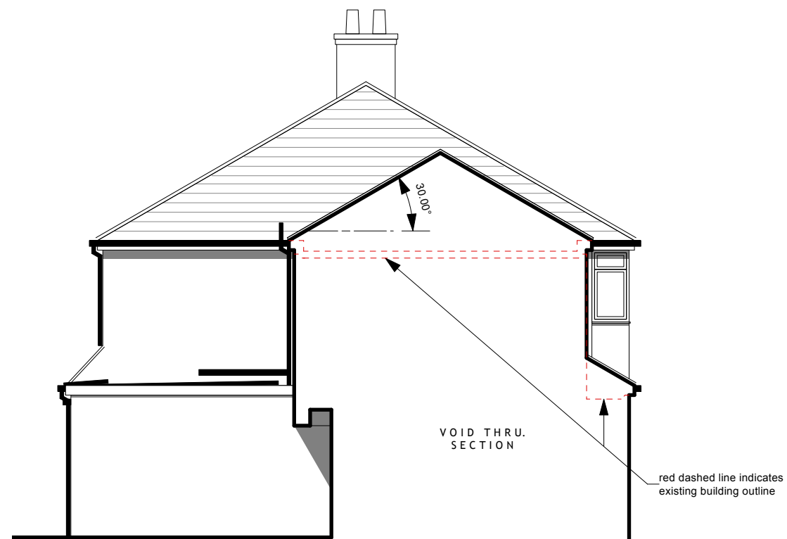
PROPOSED SIDE ELEVATION CUT ALONG PROPOSED SECTION 3
