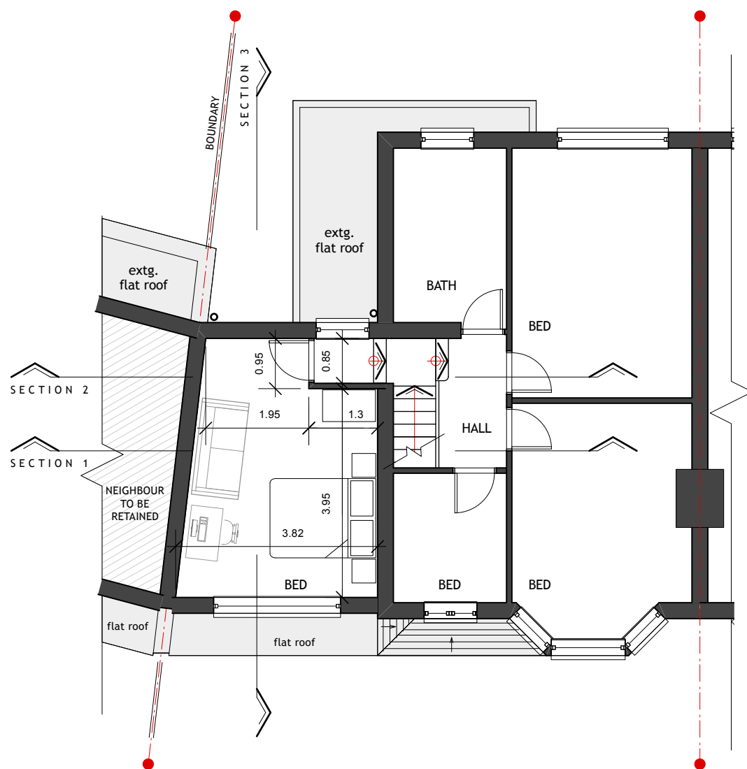
EXISTING FIRST FLOOR LAYOUT
