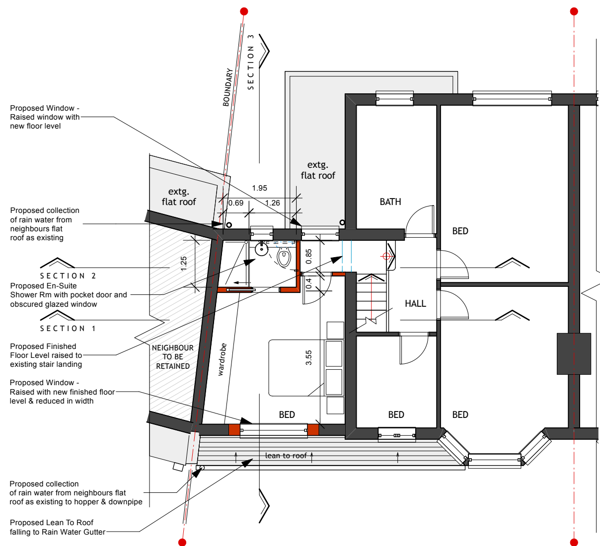
PROPOSED FIRST FLOOR LAYOUT
