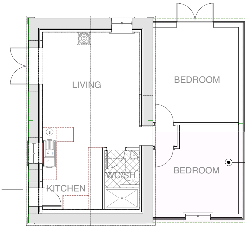
○ Floor Plan 1-100 @ A3
