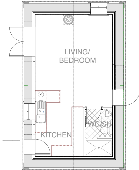
○ Floor Plan 1-100 @ A3
