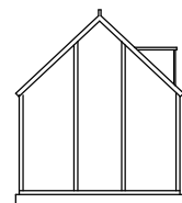
Existing Greenhouse East Elevation - 1/100
