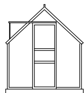
Existing Greenhouse West Elevation - 1/100
