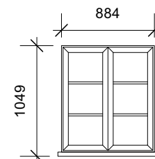
WF04 Scale 1:50
