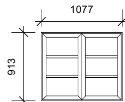
WF02 Scale 1:50
