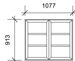
WF01 Scale 1:50
