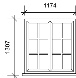
WF03 Scale 1:50
