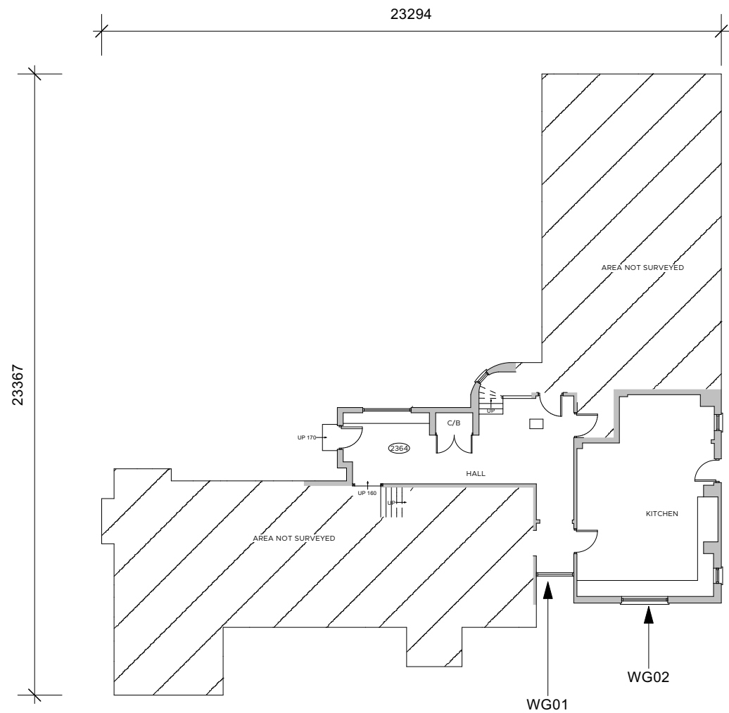
EXISTING GROUND FLOOR PLAN Scale 1:200
