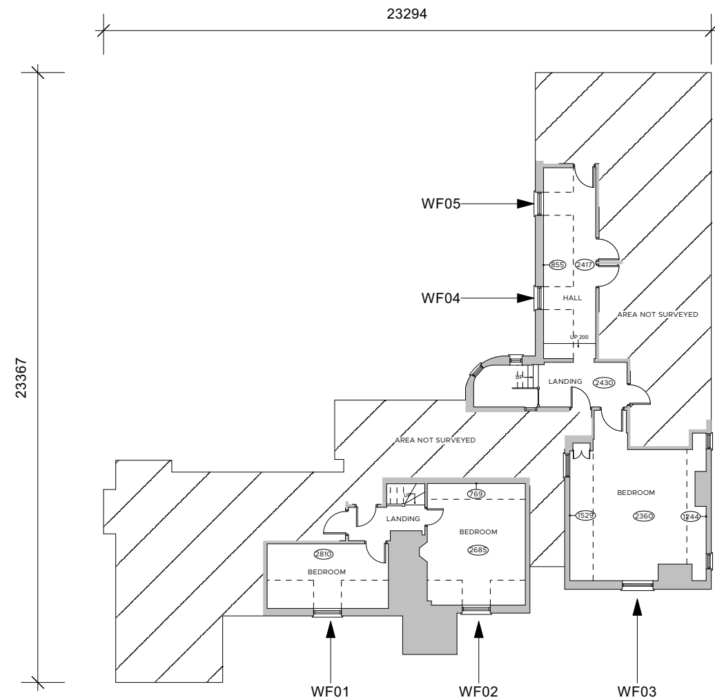
EXISTING FIRST FLOOR PLAN Scale 1:200
