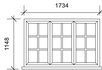
WG02 Scale 1:50
