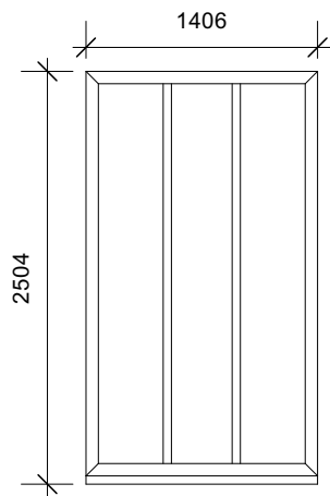
WG01 Scale 1:50
