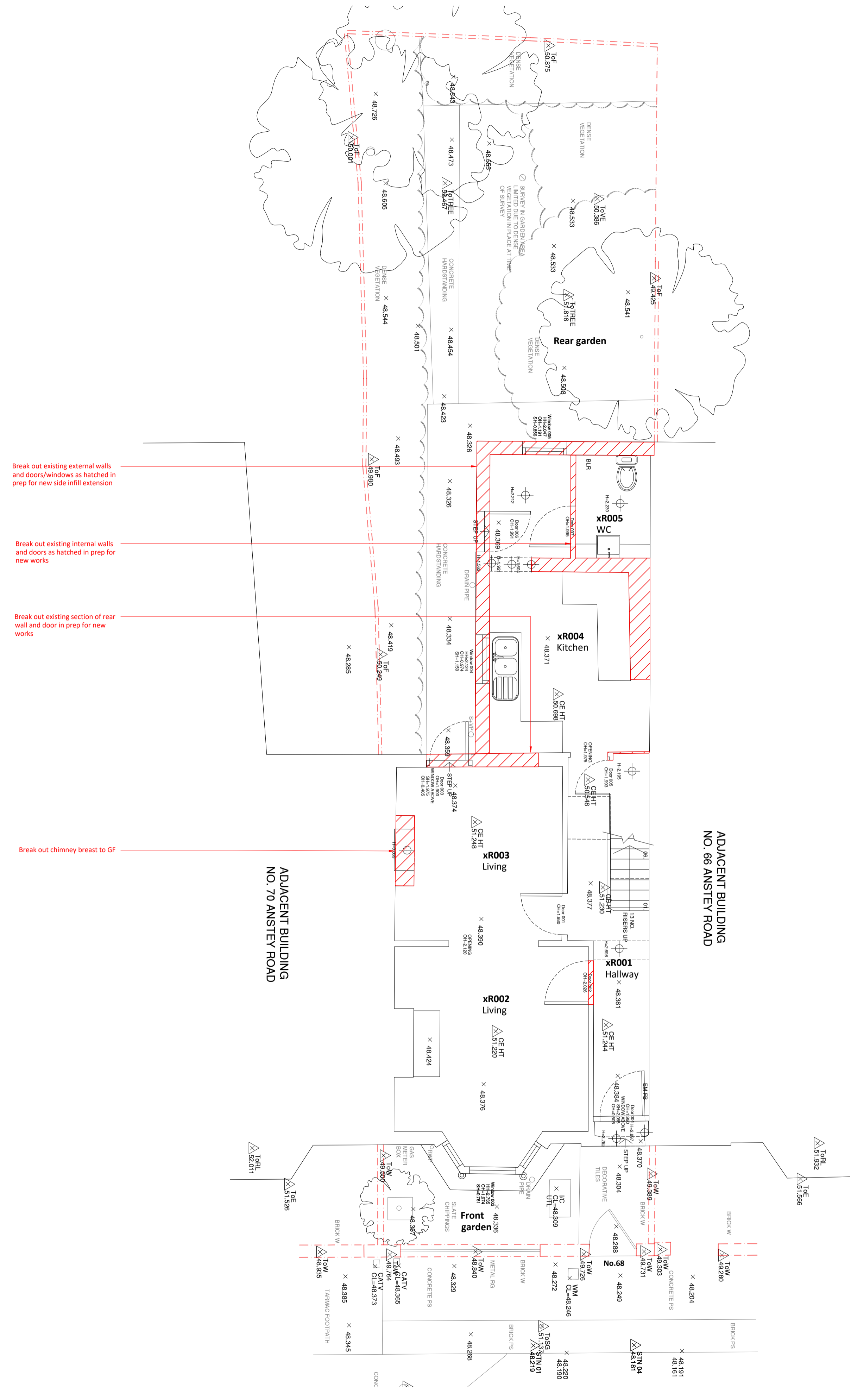
00 EXISTING GROUND FLOOR PLAN 0 0.5 1 2 3m @ A1
