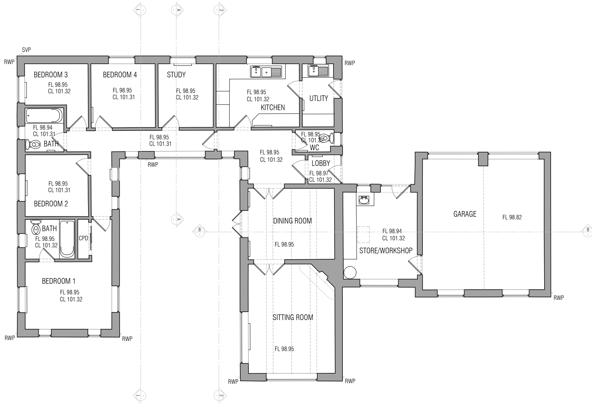
GROUND FLOOR PLAN GIA: 171.5 sqm (1846.0 sqft)
