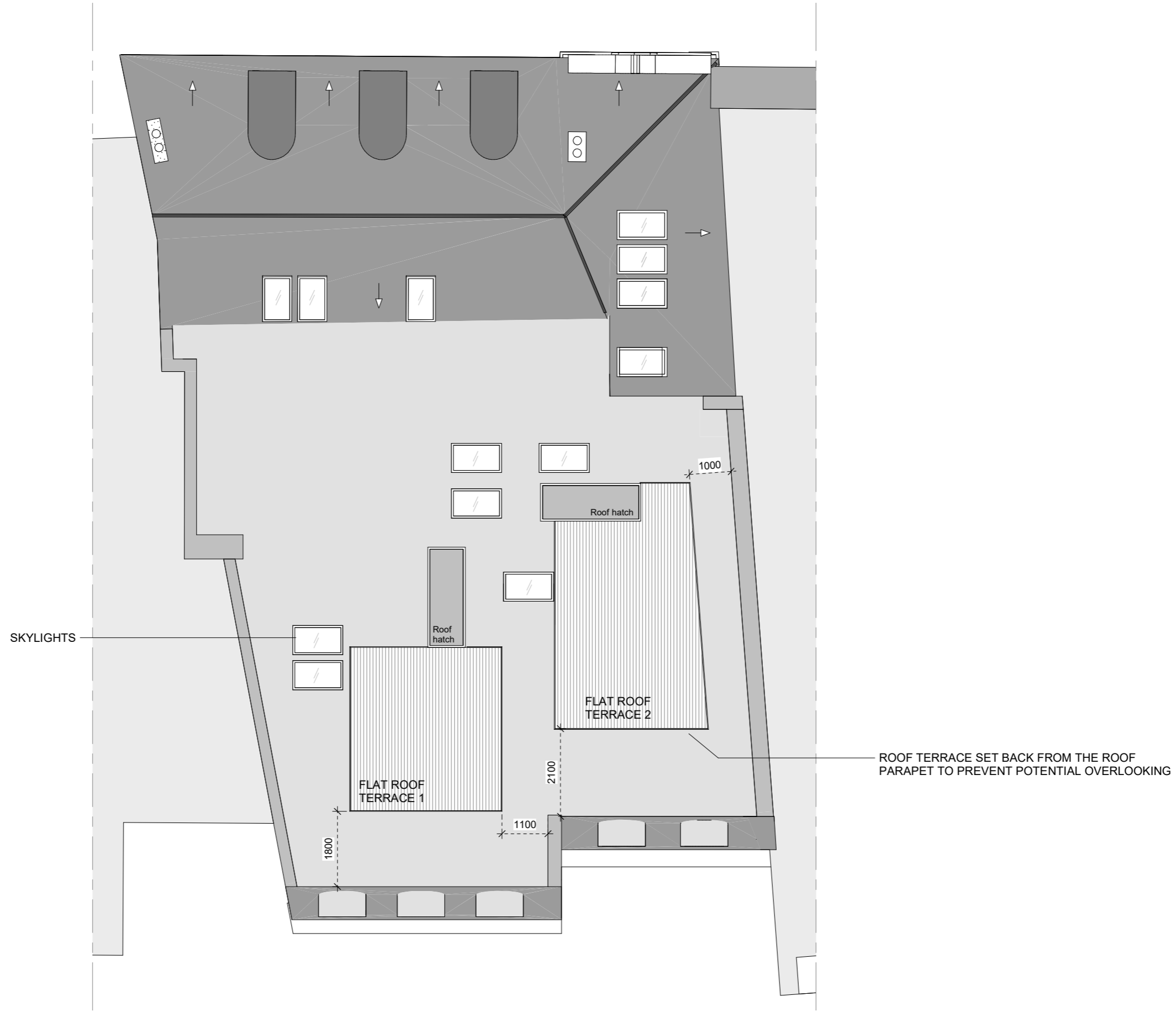
ROOF PLAN
