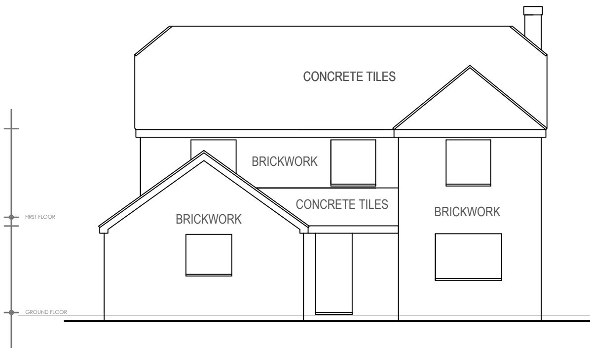
FRONT ELEVATION
