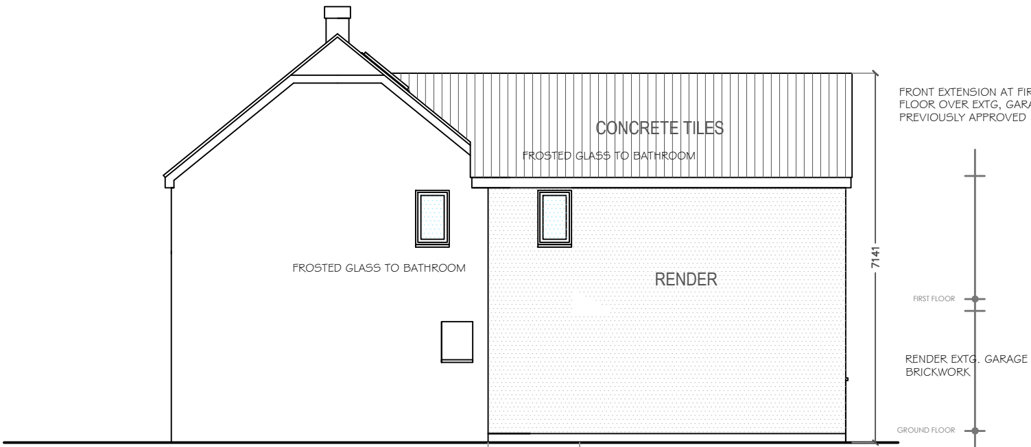
LHS ELEVATION
