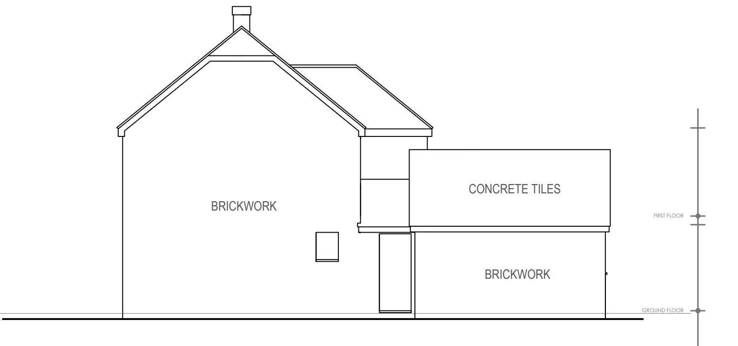
LHS ELEVATION
