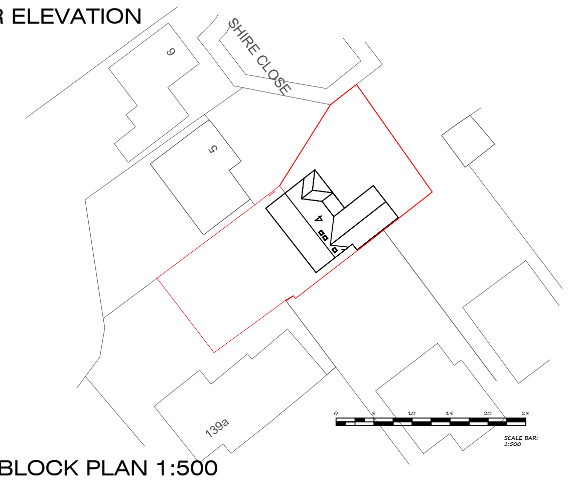
BLOCK PLAN 1:500
