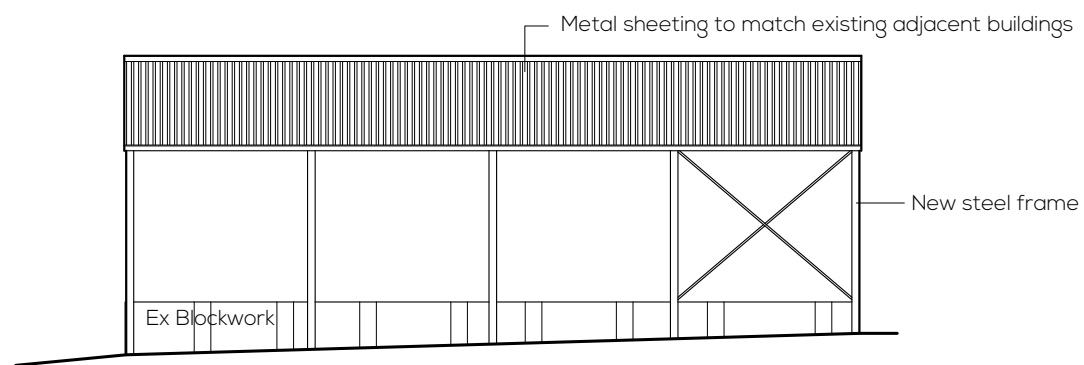
North Elevation
