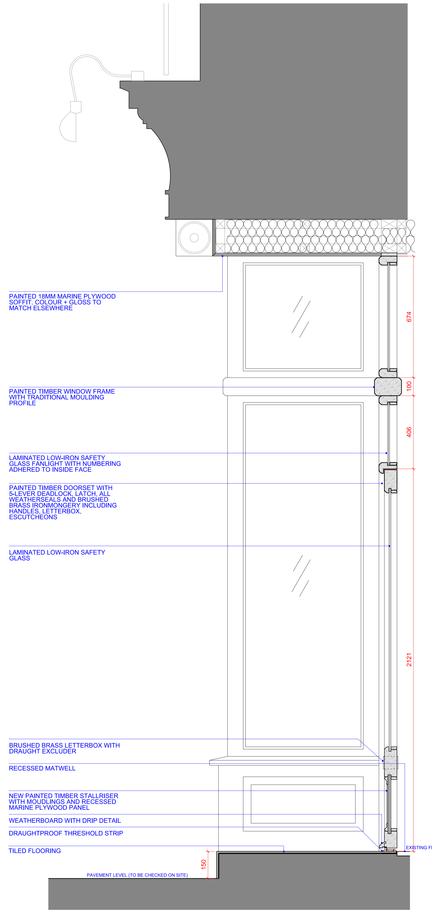
2 1:10 PROPOSED SHOPFRONT DOOR DETAIL
