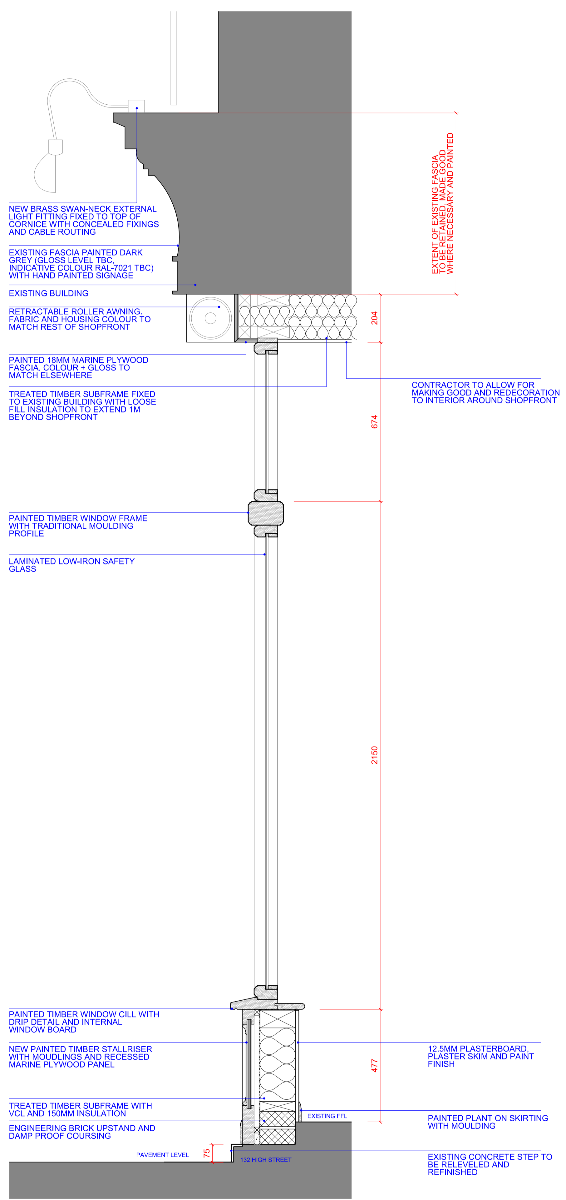
1 1:10 PROPOSED SHOPFRONT WINDOW DETAIL
