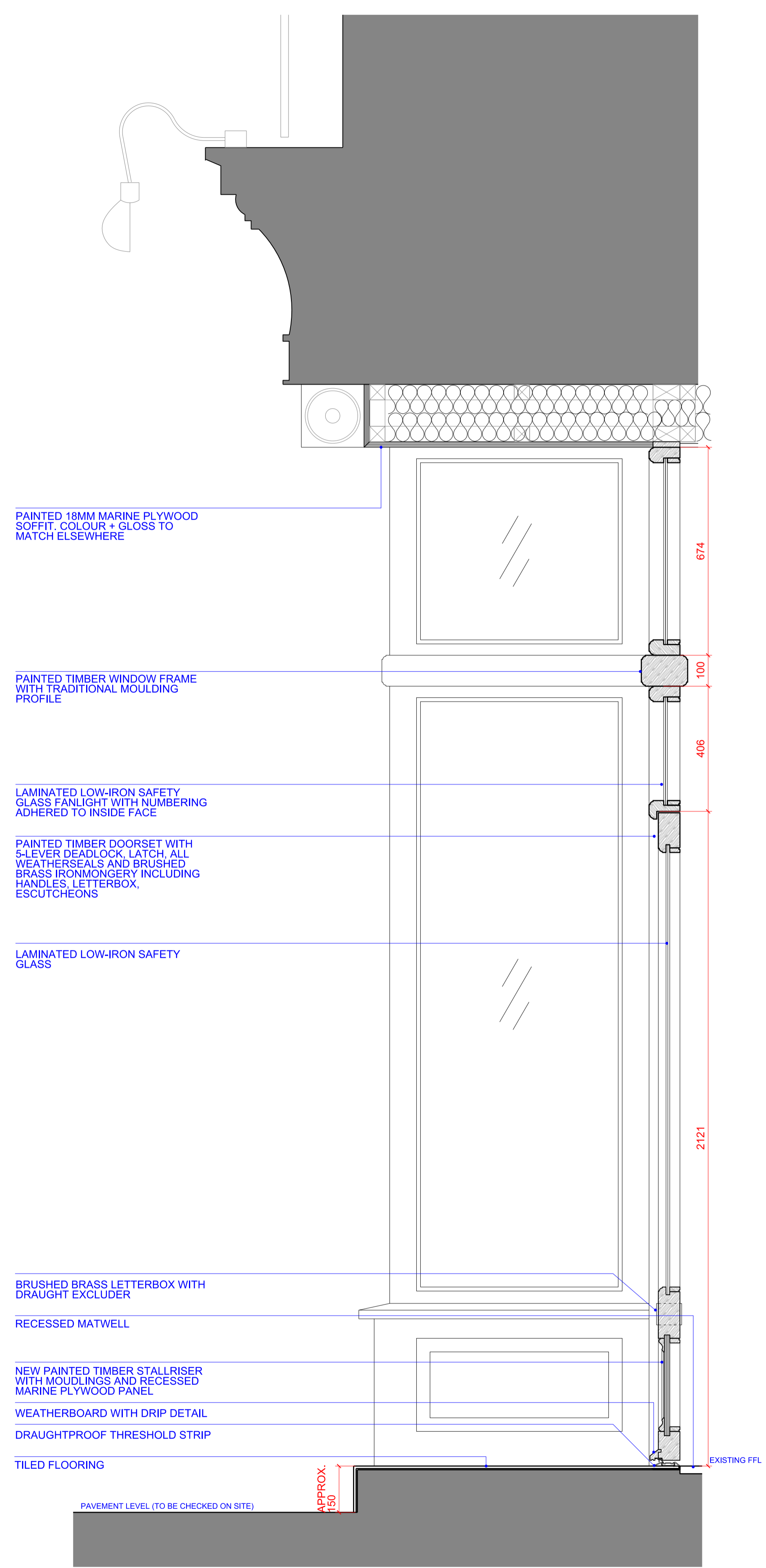
2 1:10 PROPOSED SHOPFRONT DOOR DETAIL
