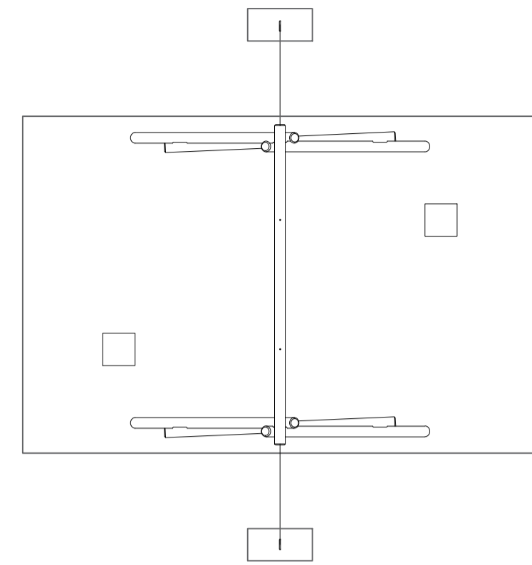
Plan View of Rope Swing with Low All Aboard
