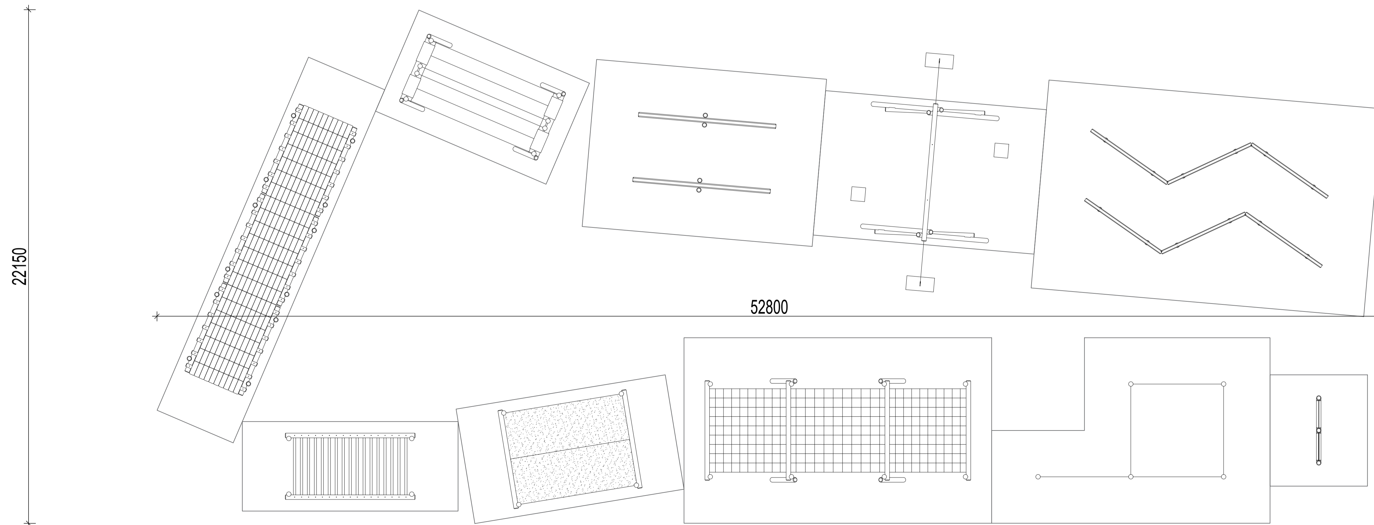
Plan View of Commando Crawl
