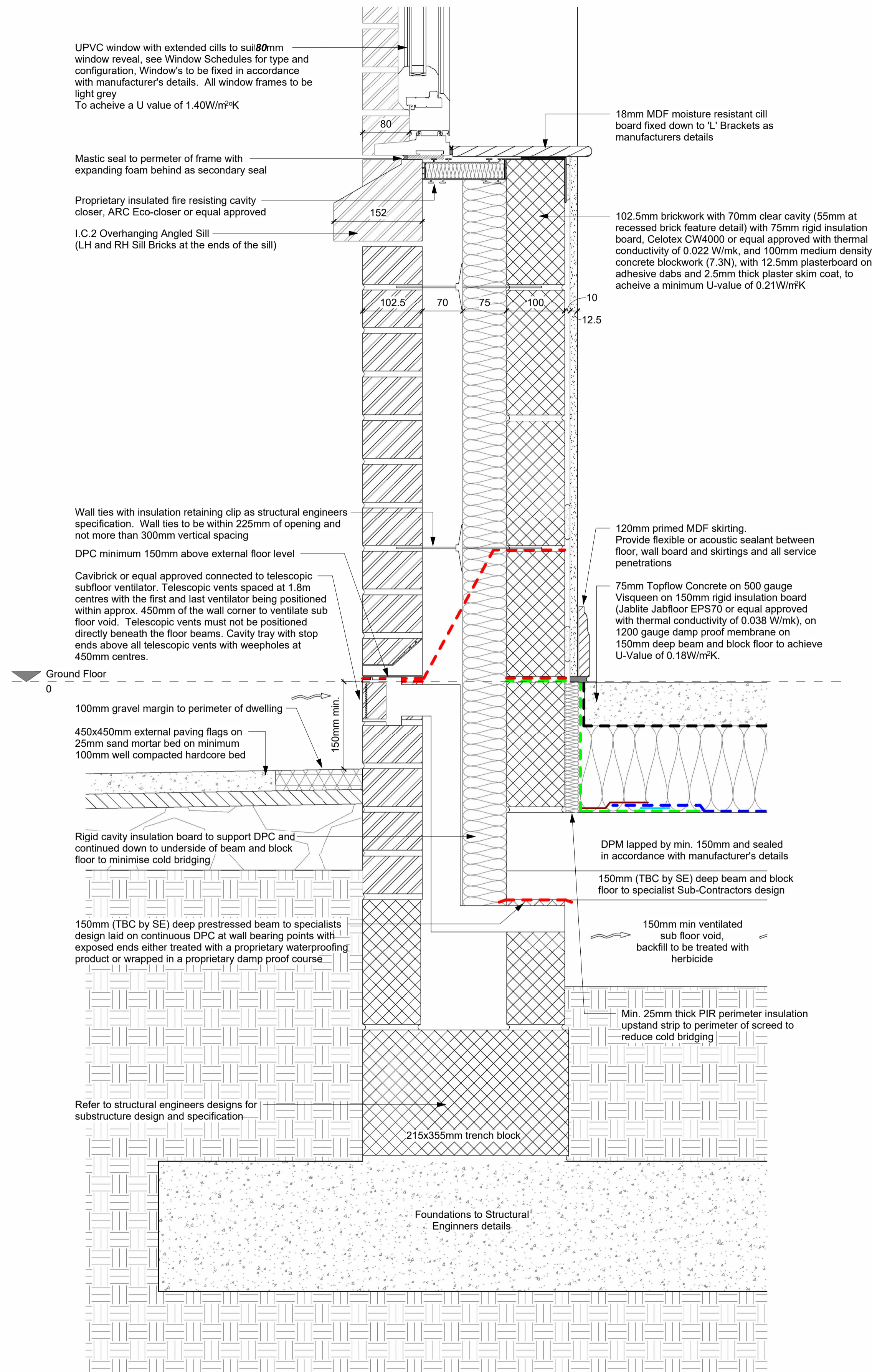
1 Typical Foundation External GL -150mm / Typical Window Cill 1:5
