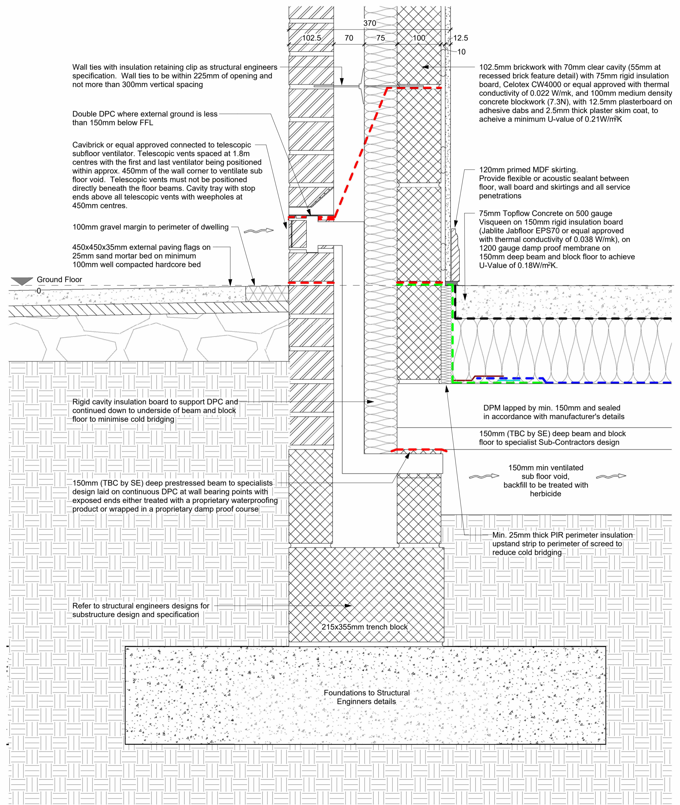
2 Typical Foundation External GL +0mm 1:5
