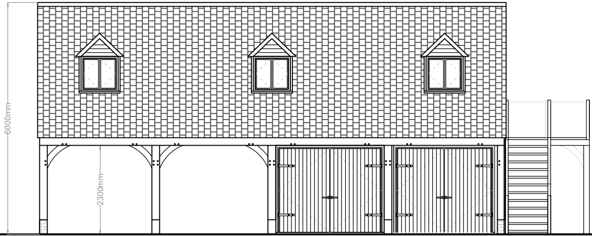
Front Elevation
