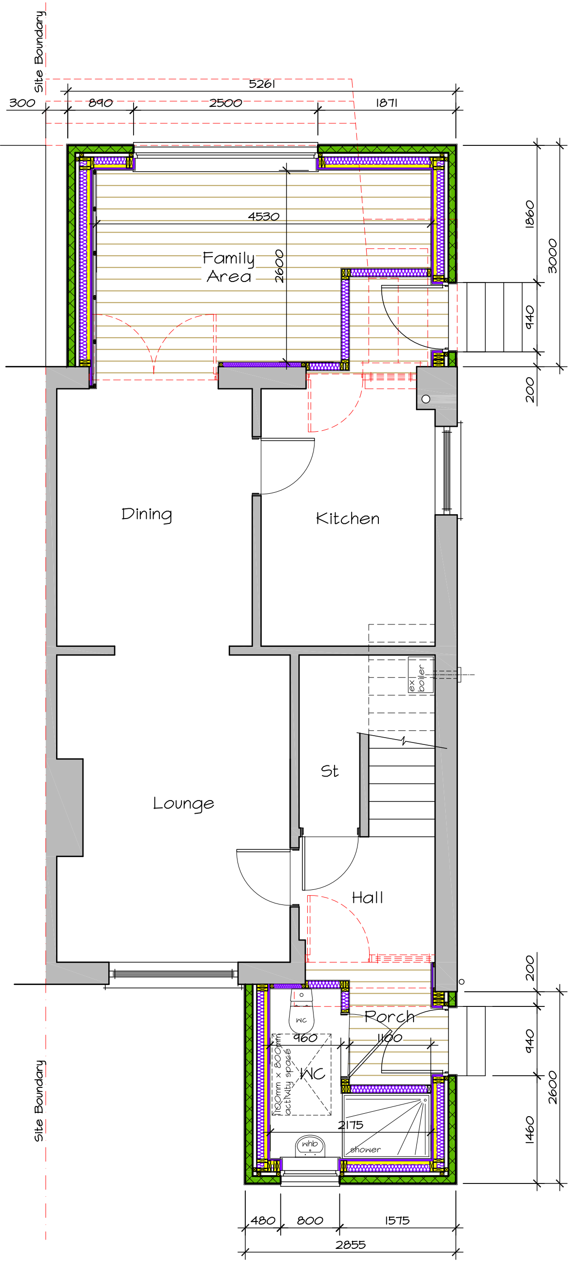
○ Proposed Ground Floor Layout Plan 1:50
