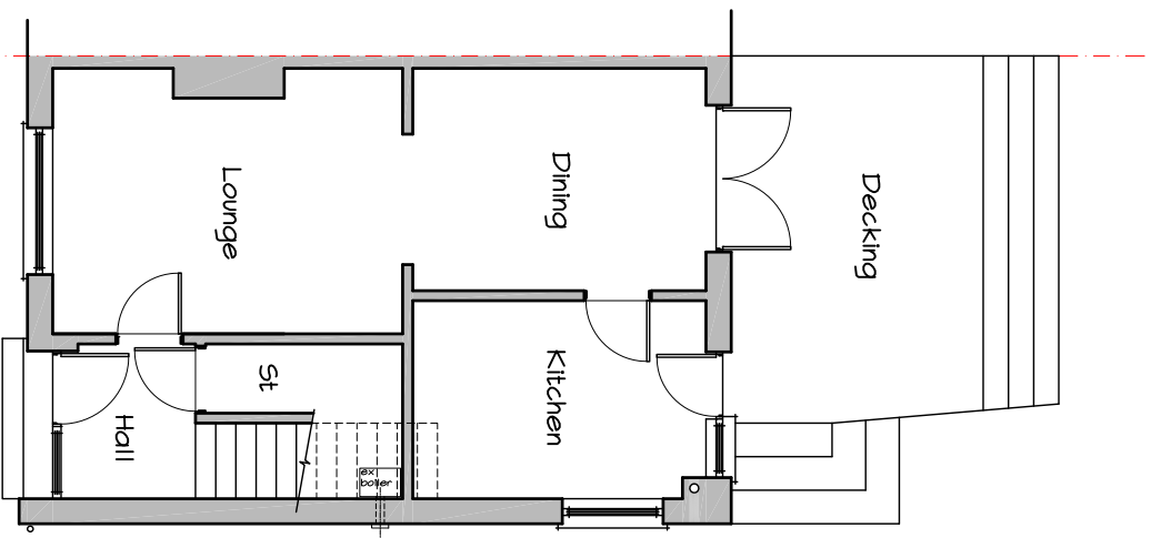
Existing Ground Floor Layout Plan 1:100
