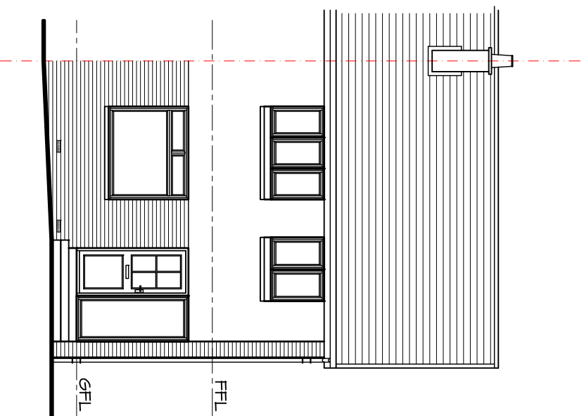
Existing South East Elevation 1:100
