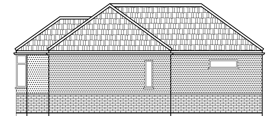
EXISTING SIDE ELEVATION-1
