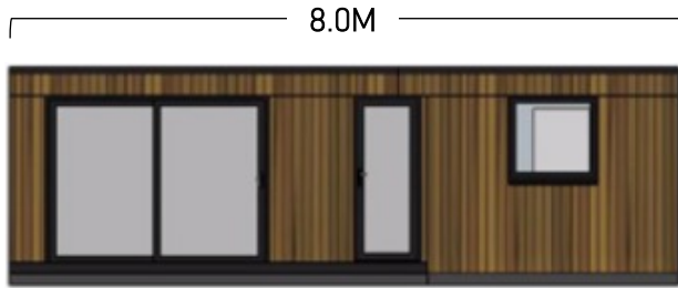
FRONT ELEVATION (EAST FACING)
