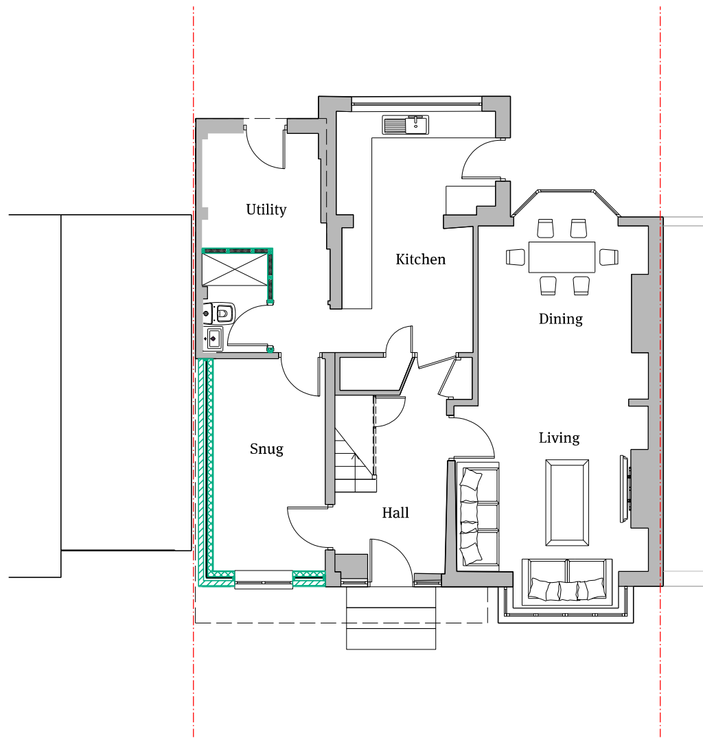
01 Ground Floor Plan 1:100 @A3
