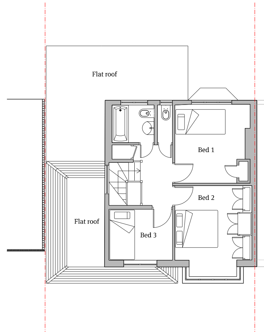
02 First Floor Plan 1:100 @A3
