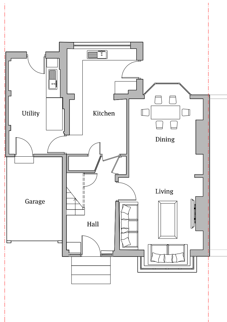
01 Ground Floor Plan 1:100 @A3
