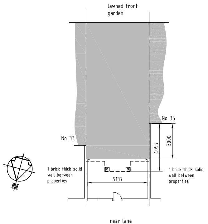
PROPOSED BLOCK PLAN SCALE 1/200
