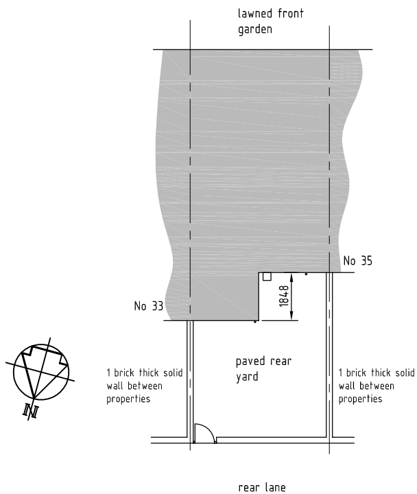
EXISTING BLOCK PLAN SCALE 1/200
