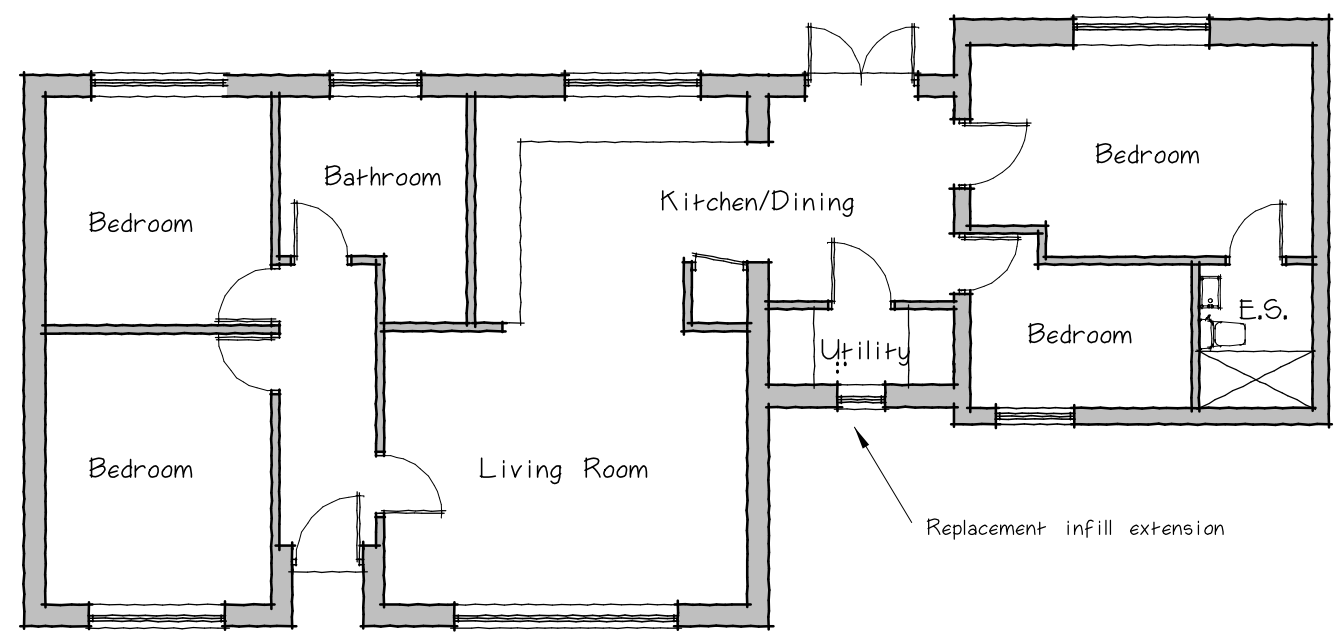
Floor Plan
