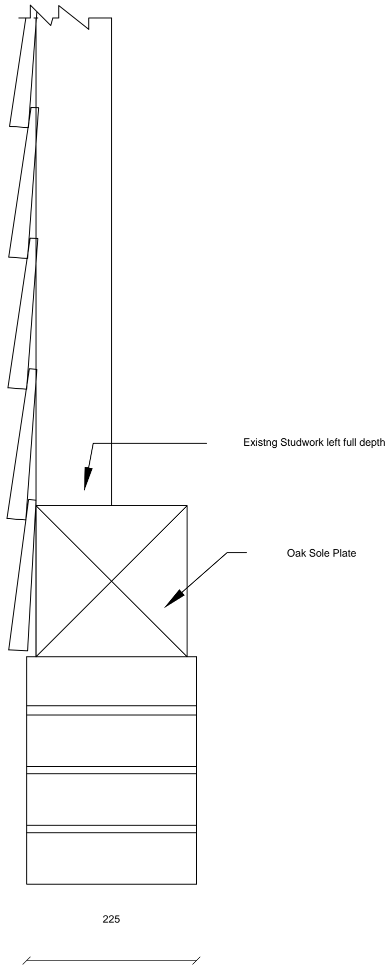
Existing Wall Construction Junction Thatched Barn Lindsey Scale 1:5
