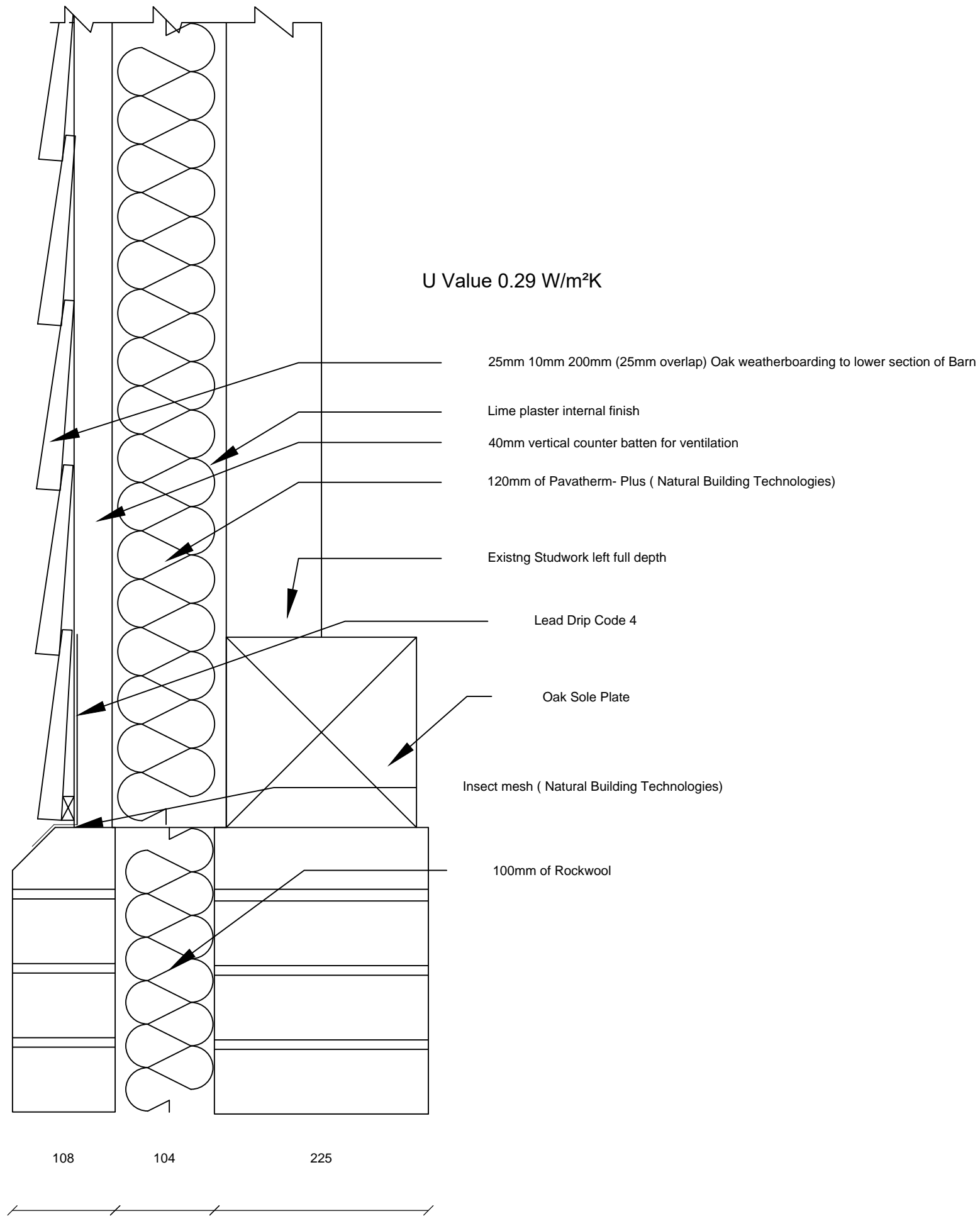
Wall Construction Junction with Eaves Thatched Barn Lindsey Scale 1:5
