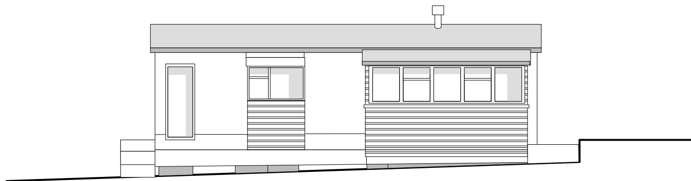
Front West Elevation
