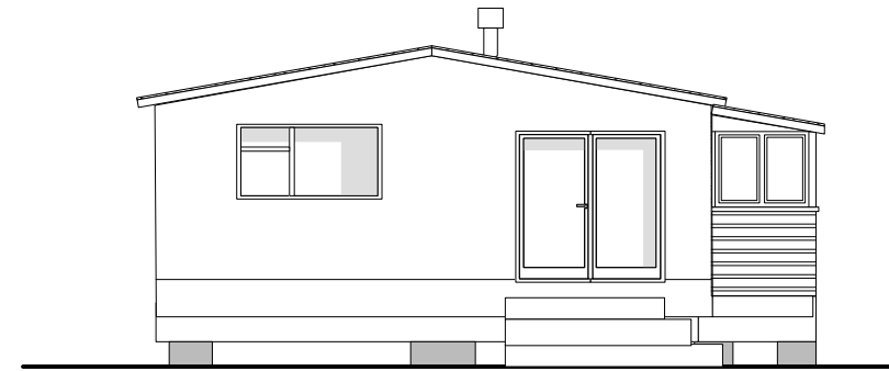
Left North Gable Elevation
