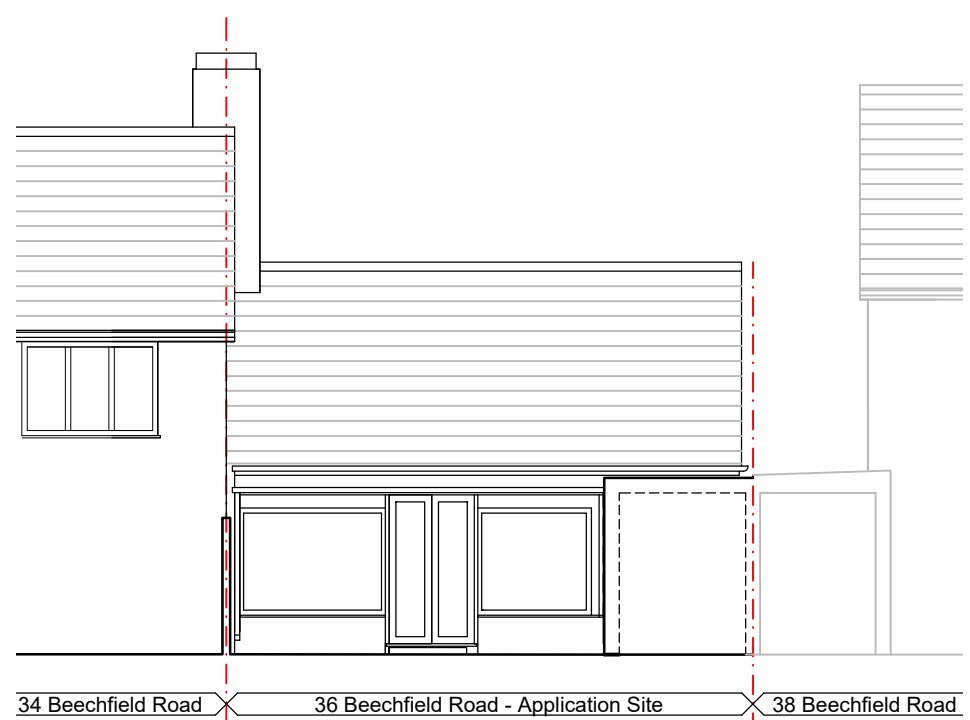
Rear Elevation
