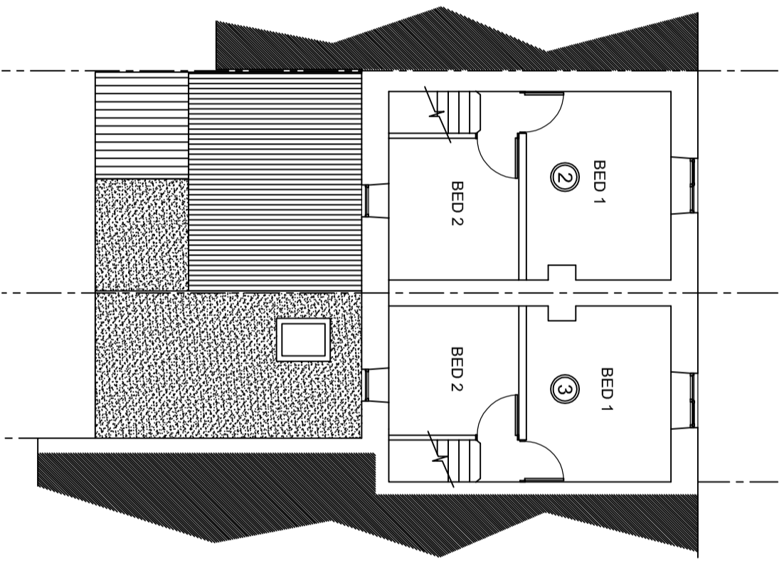
FIRST FLOOR
