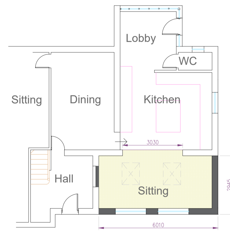
Part Ground Floor Plan
