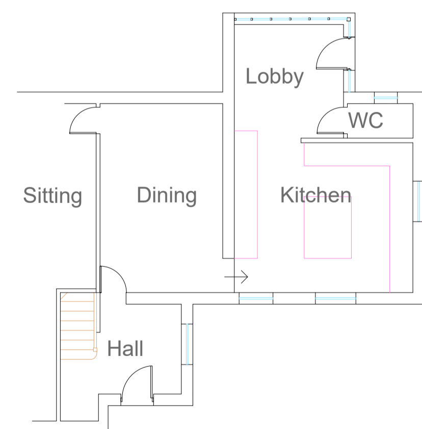
Part Ground Floor Plan
