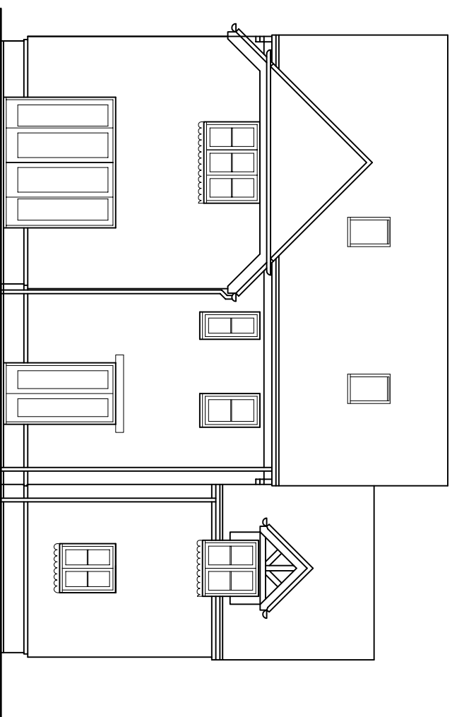
EAST ELEVATION
