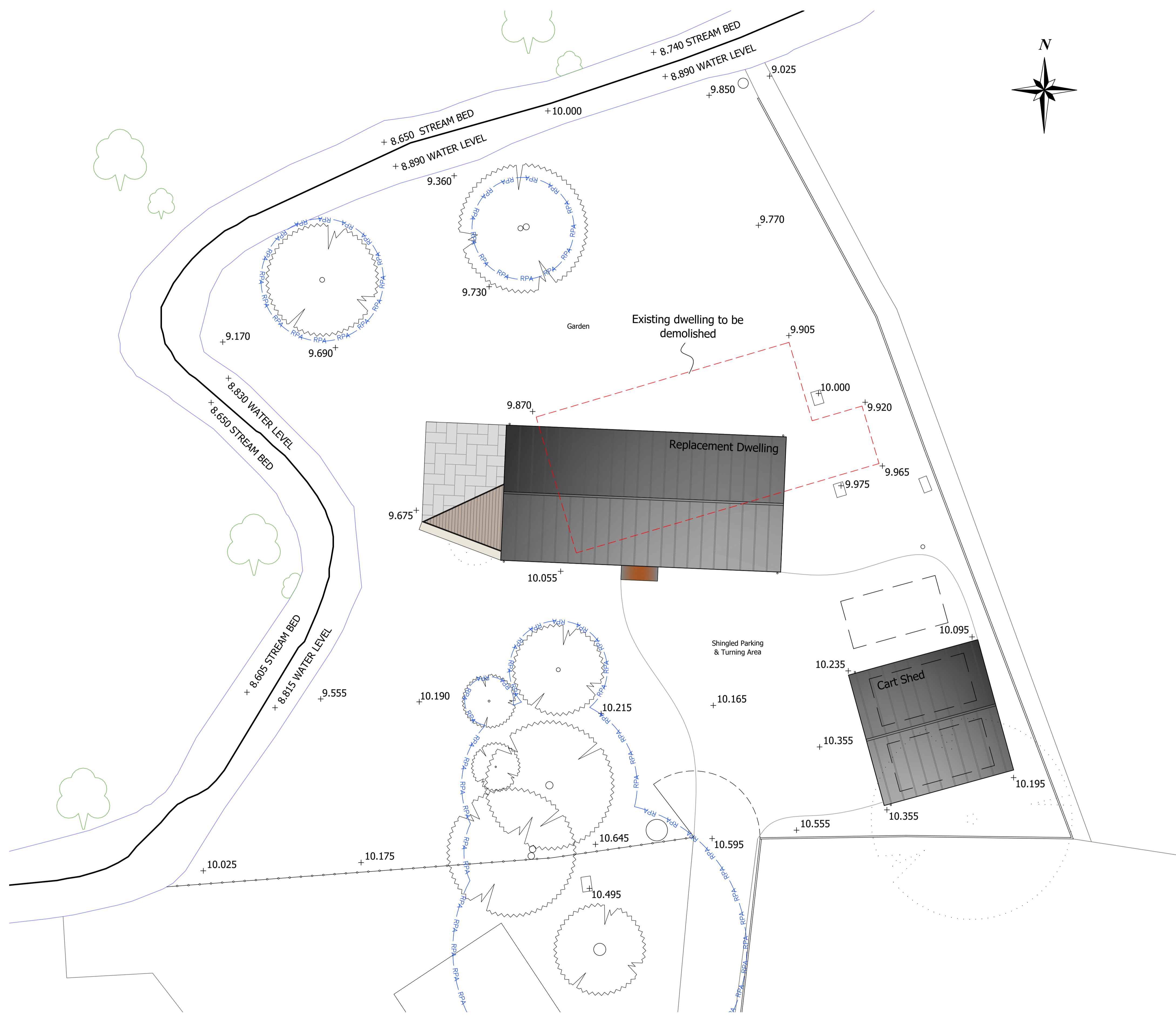
Part Site Plan 1:100 0 1 5m
