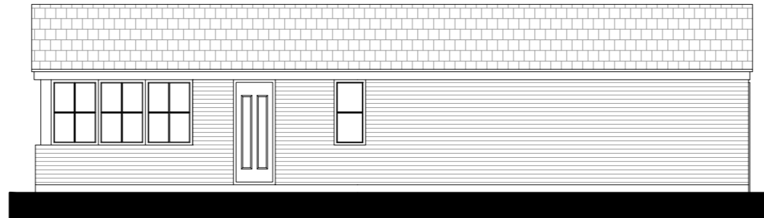
EAST ELEVATION | PROPOSED 0m 1.0m 2.5m 5.0m 1:100
