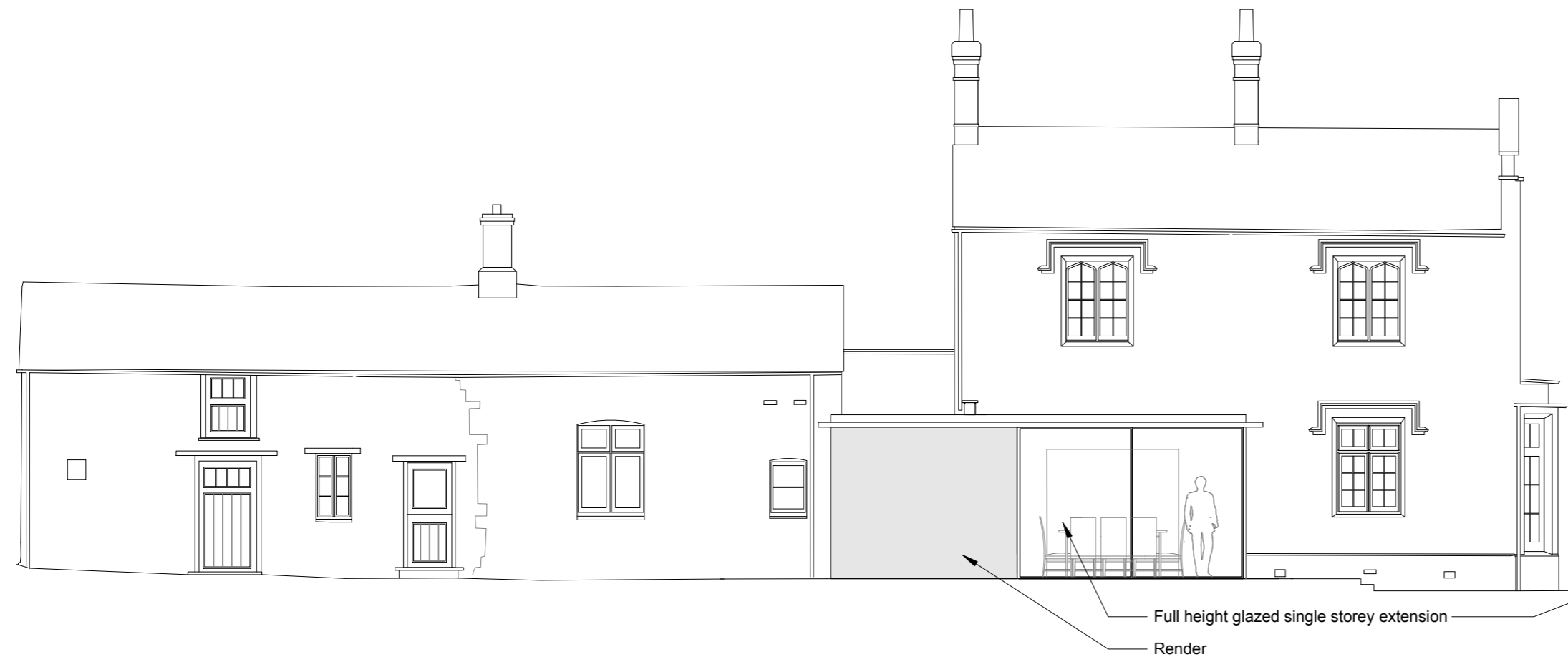
03 PROPOSED NORTH ELEVATION
