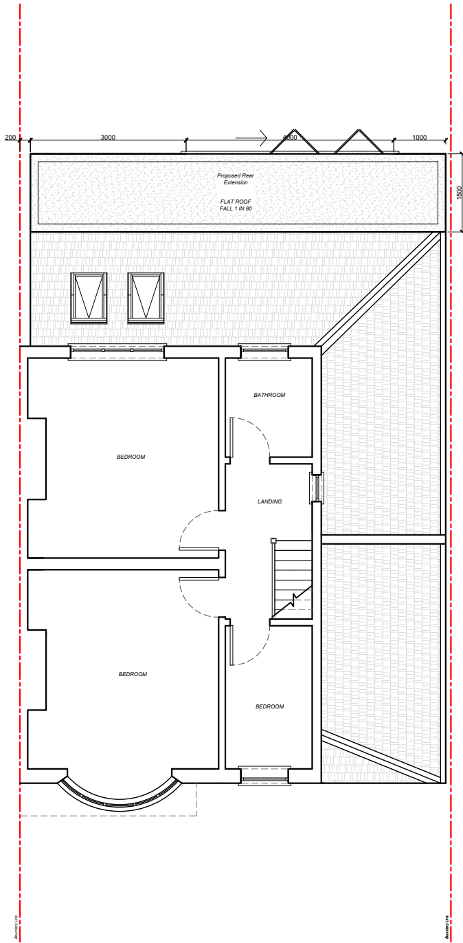
Proposed First Floor Plan (Scale 1:100)
