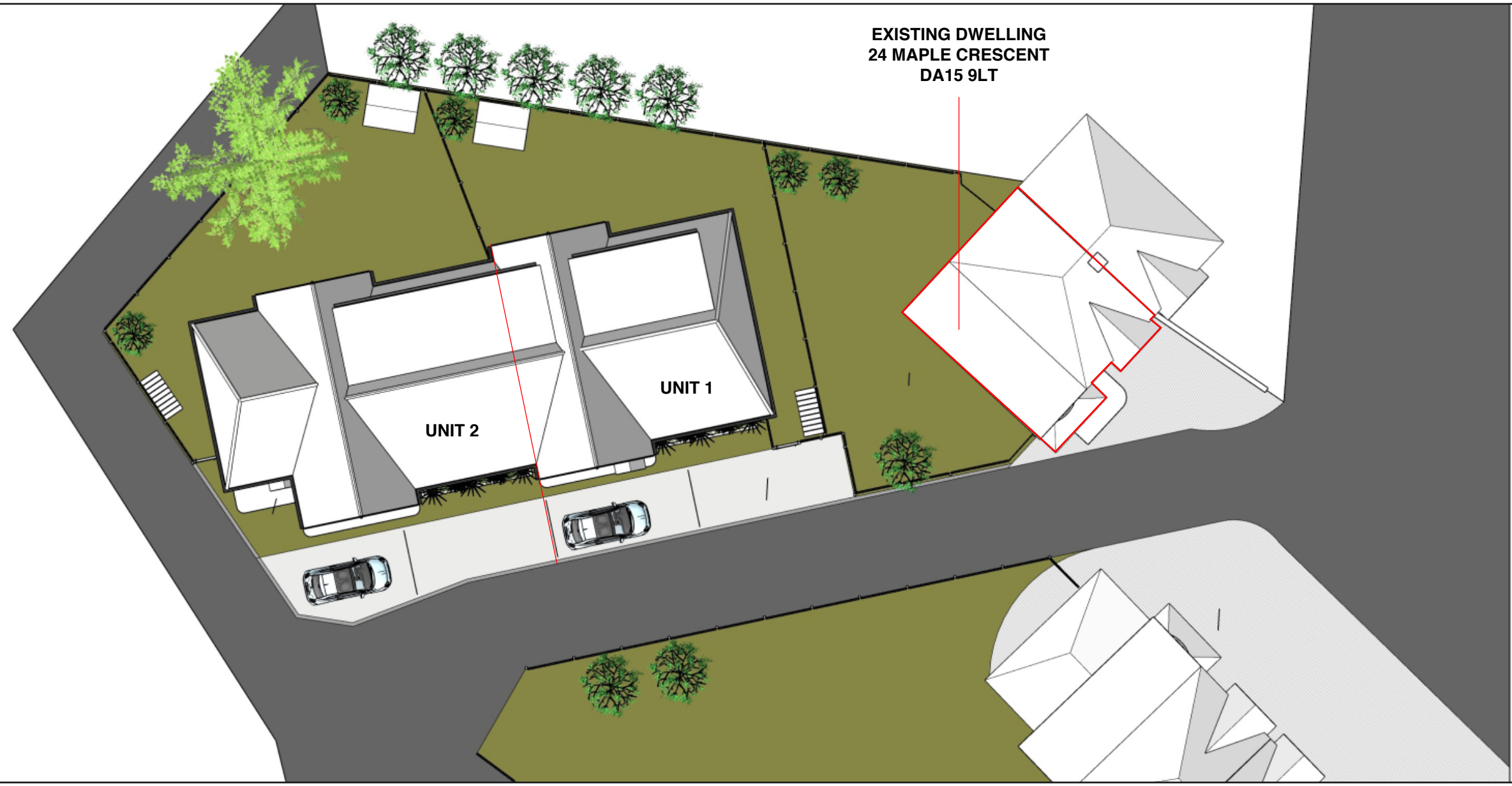
MAPLE CRESCENT BUNGALOW MASSING SCHEME - SITE PLAN
