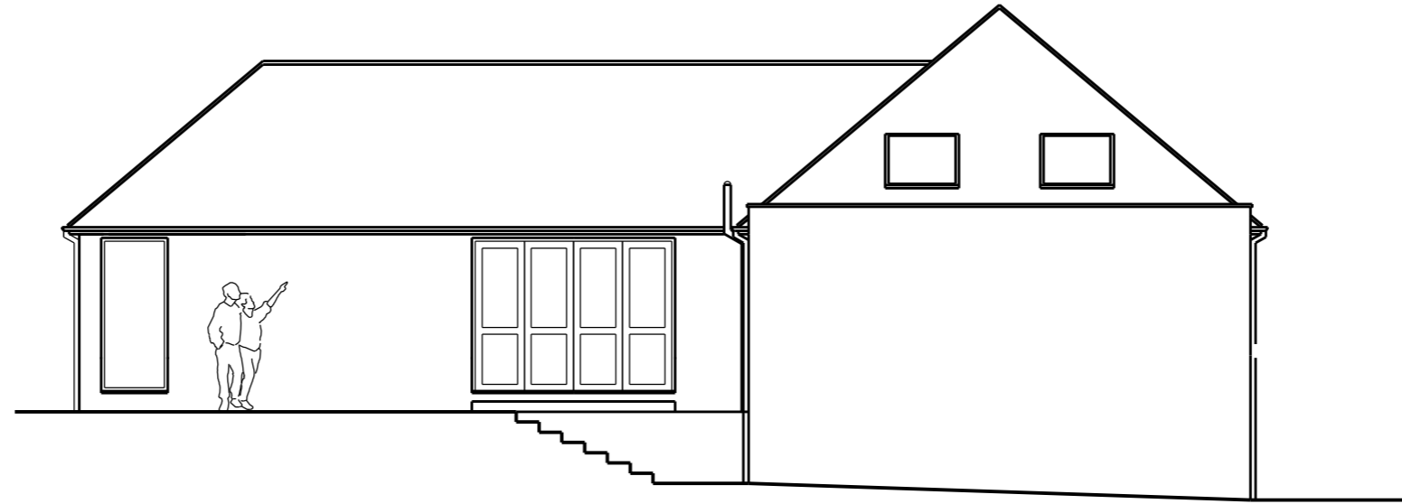
SIDE ELEVATION FACING No 114 PARK HILL ROAD
