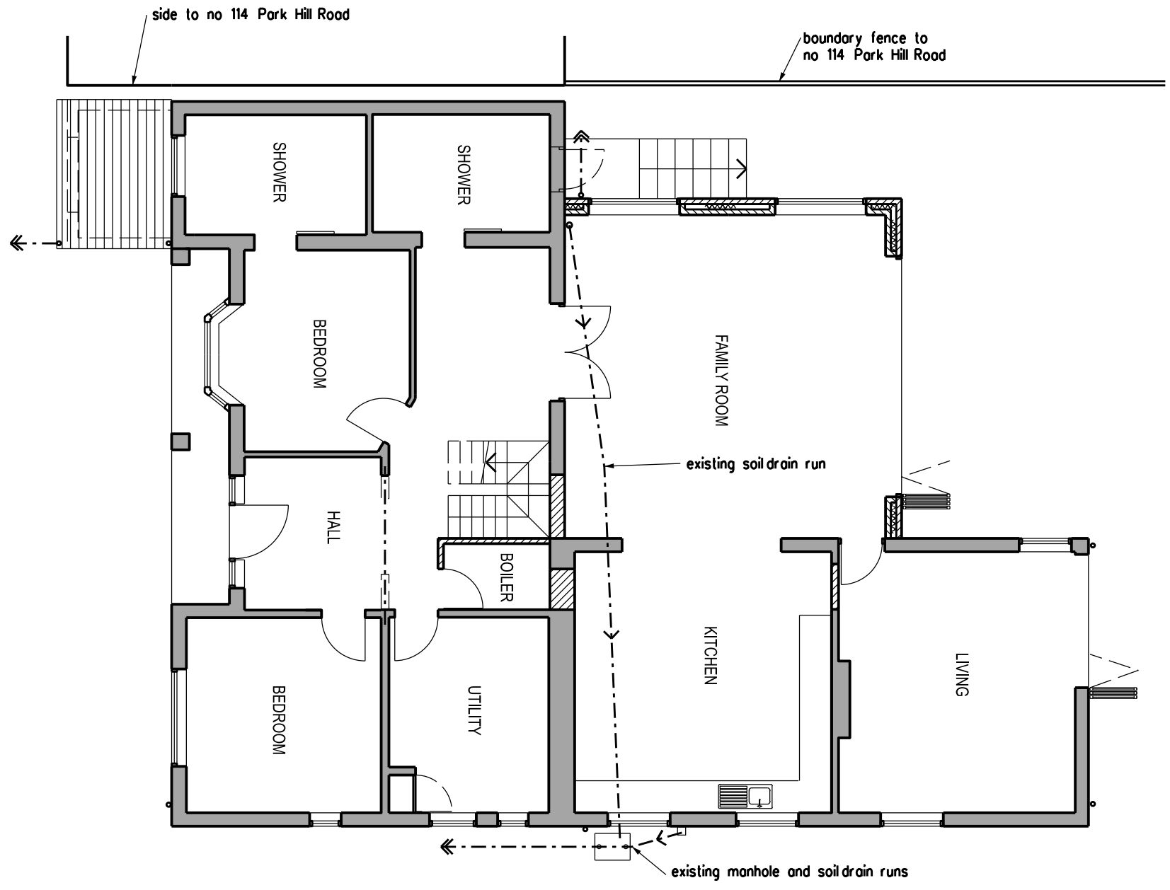
GROUND FLOOR PLAN SEE 1:50 SCALE DRG Nos RP/08 & RP/09
