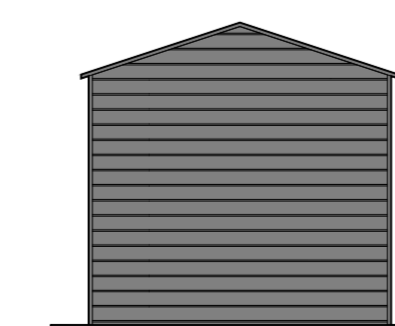
SOUTH-EAST ELEVATION
