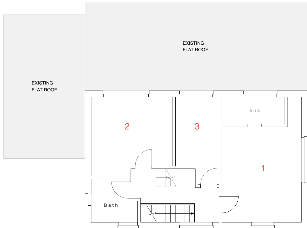
Existing First Floor Plan at 1:100 scale
