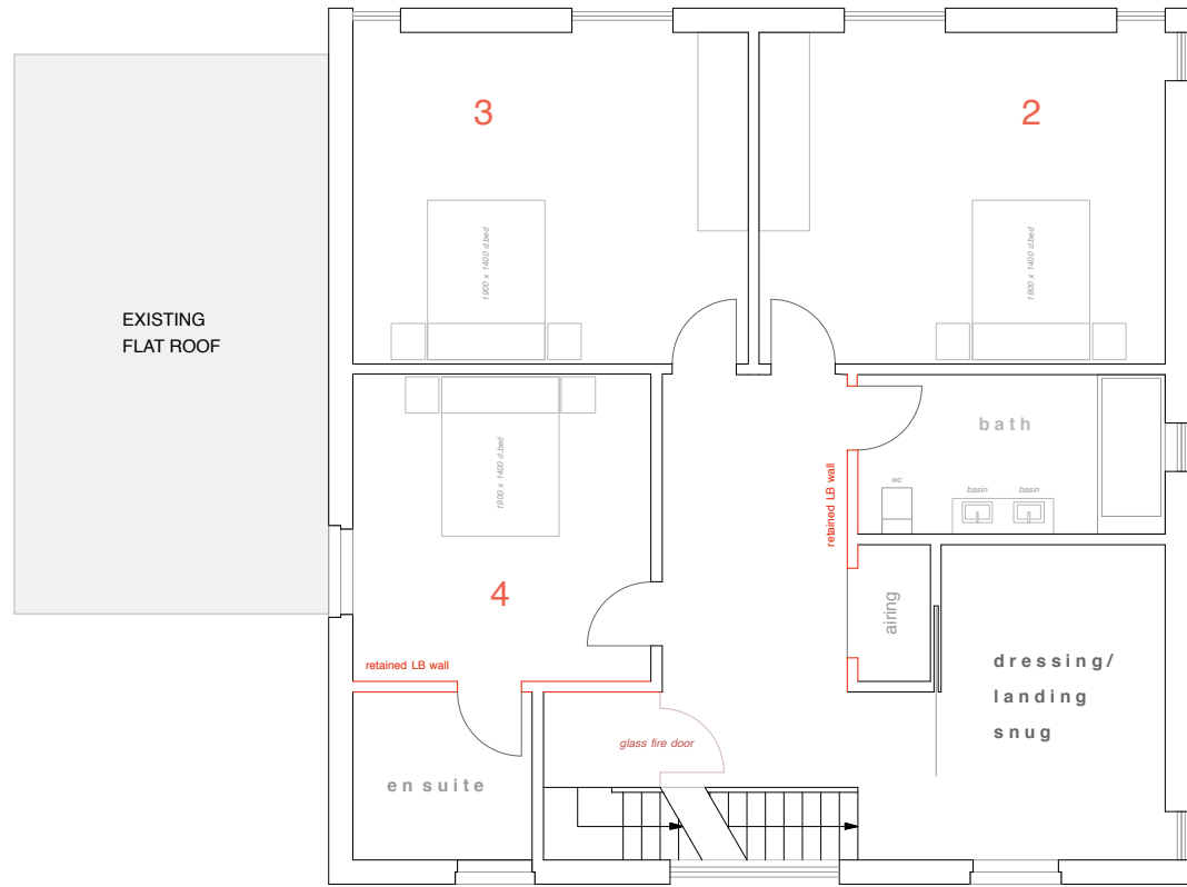
Proposed First Floor Plan at 1:100 scale
