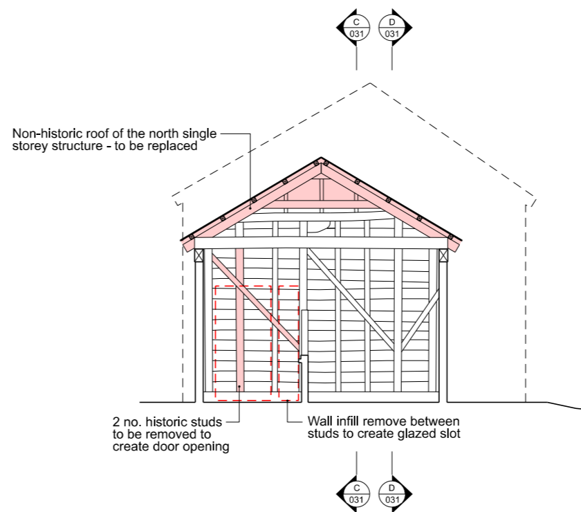
Section GG - north single storey structure
