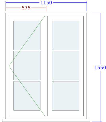
2. Flush Casement Window (FF Rear Harry's Bed)
