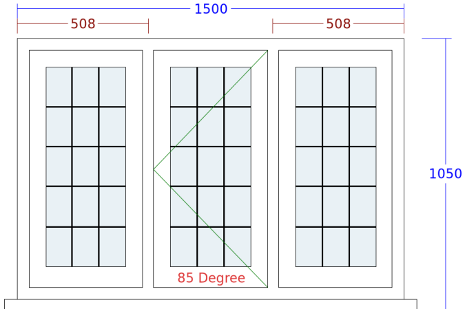
4. Flush Casement Window (FF Rear Main Bed)
