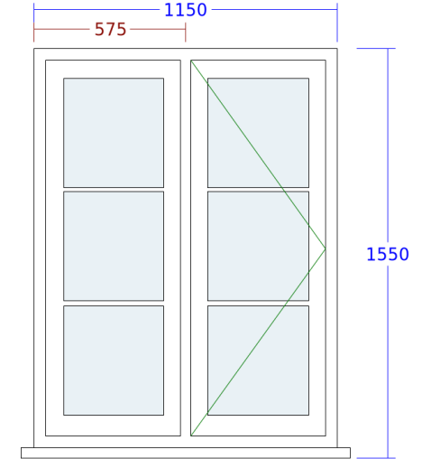
3. Flush Casement Window (FF Rear Bathroom)
