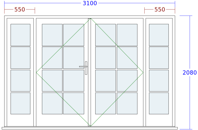
1. French Door (GF Rear)
