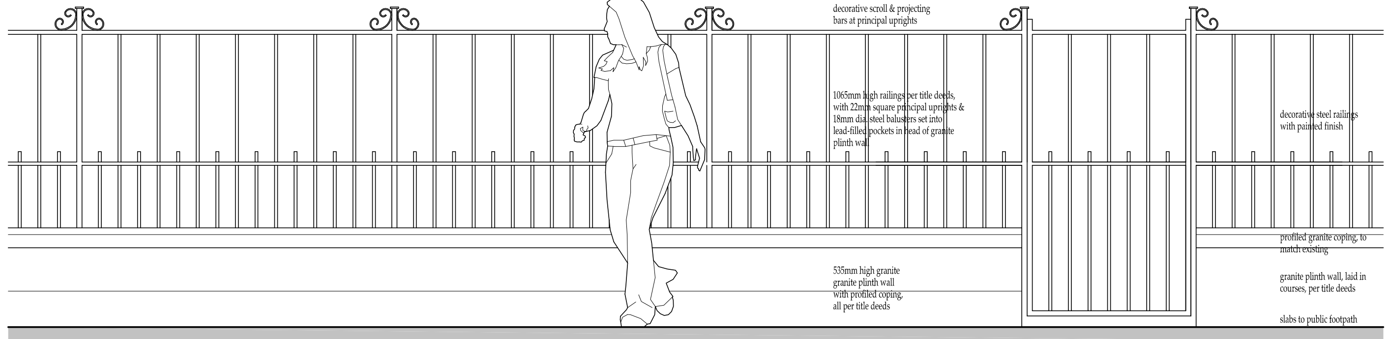
PROFILE OF NEW RAILINGS TO GARDEN GROUND: AS PROPOSED Scale 1:20 at A3
