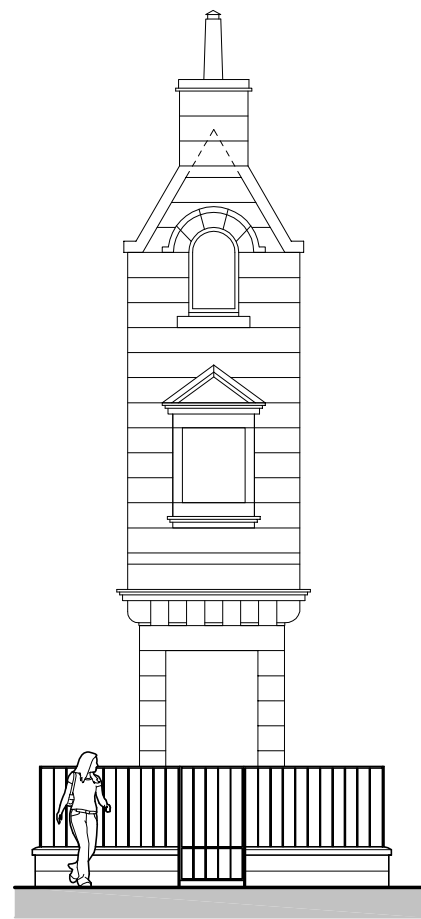
SOUTH-EAST ELEVATION: AS PROPOSED Scale 1:100 at A3
