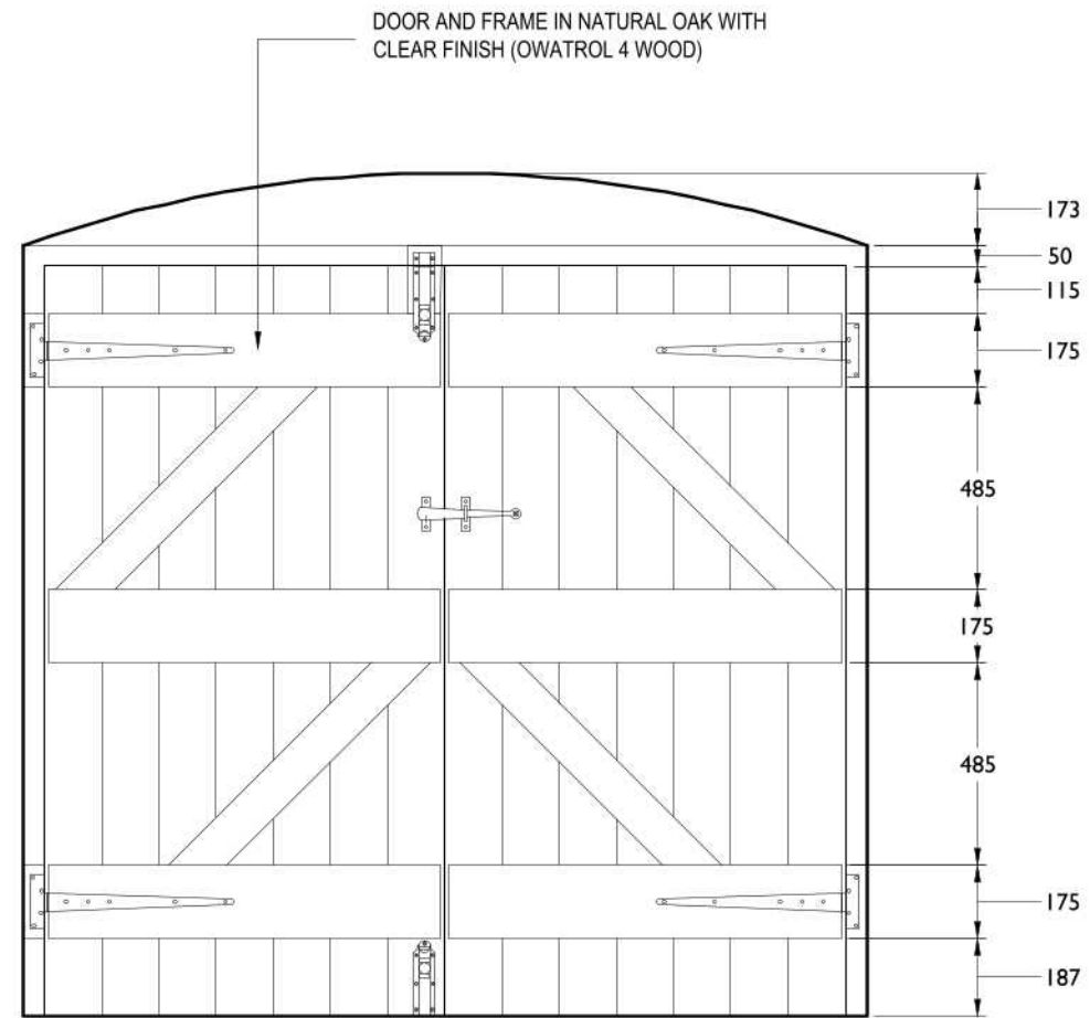
INNER ELEVATION
