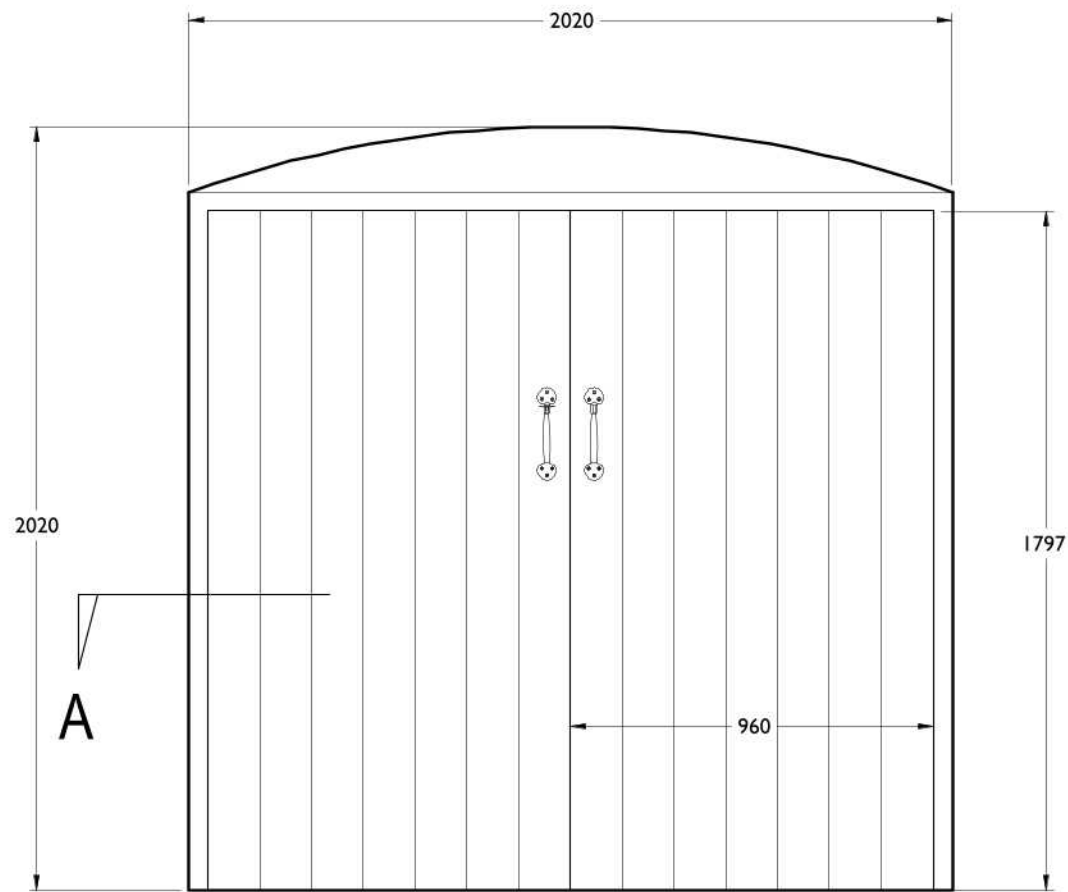
OUTER ELEVATION
