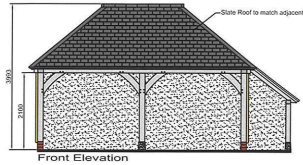
Front Elevation
