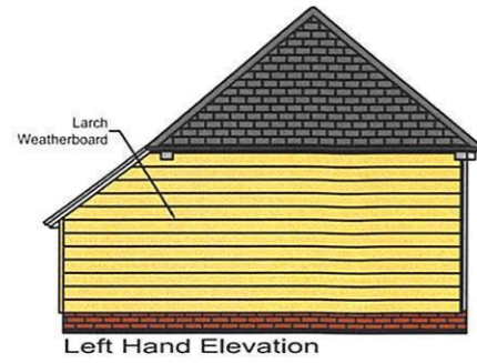
Left Hand Elevation
